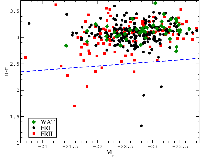
Fig. 6. u - r color vs. absolute r -band magnitude, M_r , for the WATCAT FRICAT and FRIICAT hosts. Shown are WATs (green diamonds), FR Is (black dots), and FR IIs (red squares). WATs are associated with red ETGs. The dashed blue line represents the relation from Schawinski et al. (2009) that separates red and blue early-type galaxies.
