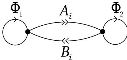
Figure 1. The \mathcal{A}_1 quiver.
