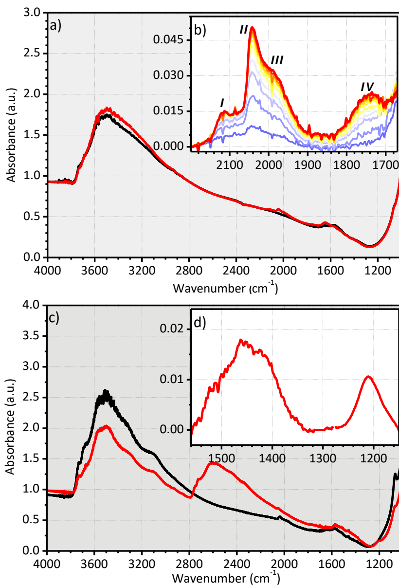
Figure 3. Part a): FT-IR spectra of the Pt/Al_2O_3 catalyst before (black) and after (red) the reduction step, accomplished in a H_2/N_2 flow (10% H_2 , 20 mL/min). Part b): magnification of the 2200-1700\text{ cm}^{-1} range, where linear Pt-hydrides contribute to the spectra. The spectra in part b) are reported after subtraction of the spectrum prior reduction (black curve in part a). Part c) FT-IR spectra of the Pt/Al_2O_3 catalyst after the reduction step (black), and the effect of dosing D_2 (red). The spectrum in part d) is the difference between the two.
