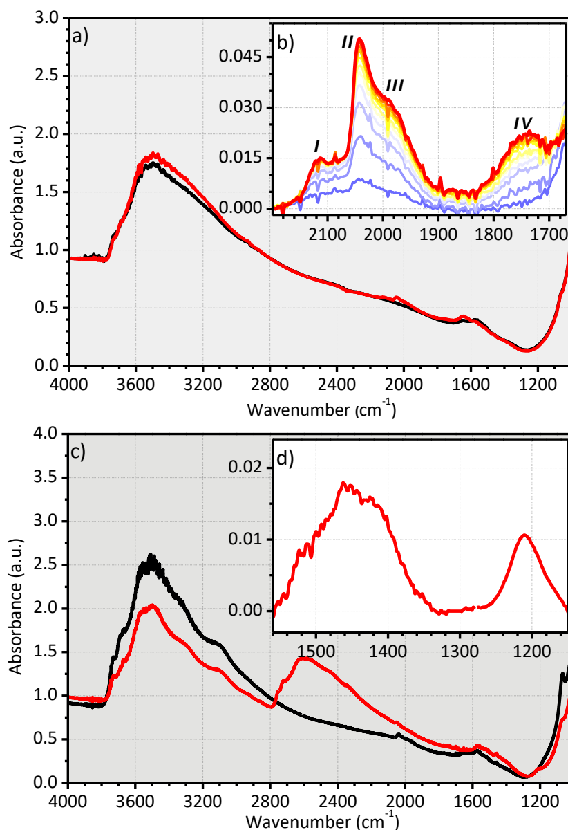
Figure 3. Part a): FT-IR spectra of the \text{Pt}/\text{Al}_2\text{O}_3 catalyst before (black) and after (red) the reduction step, accomplished in a \text{H}_2/\text{N}_2 flow (10% \text{H}_2 , 20 mL/min). Part b): magnification of the 2200\text{--}1700\text{ cm}^{-1} range, where linear Pt-hydrides contribute to the spectra. The spectra in part b) are reported after subtraction of the spectrum prior reduction (black curve in part a). Part c) FT-IR spectra of the \text{Pt}/\text{Al}_2\text{O}_3 catalyst after the reduction step (black), and the effect of dosing \text{D}_2 (red). The spectrum in part d) is the difference between the two.
