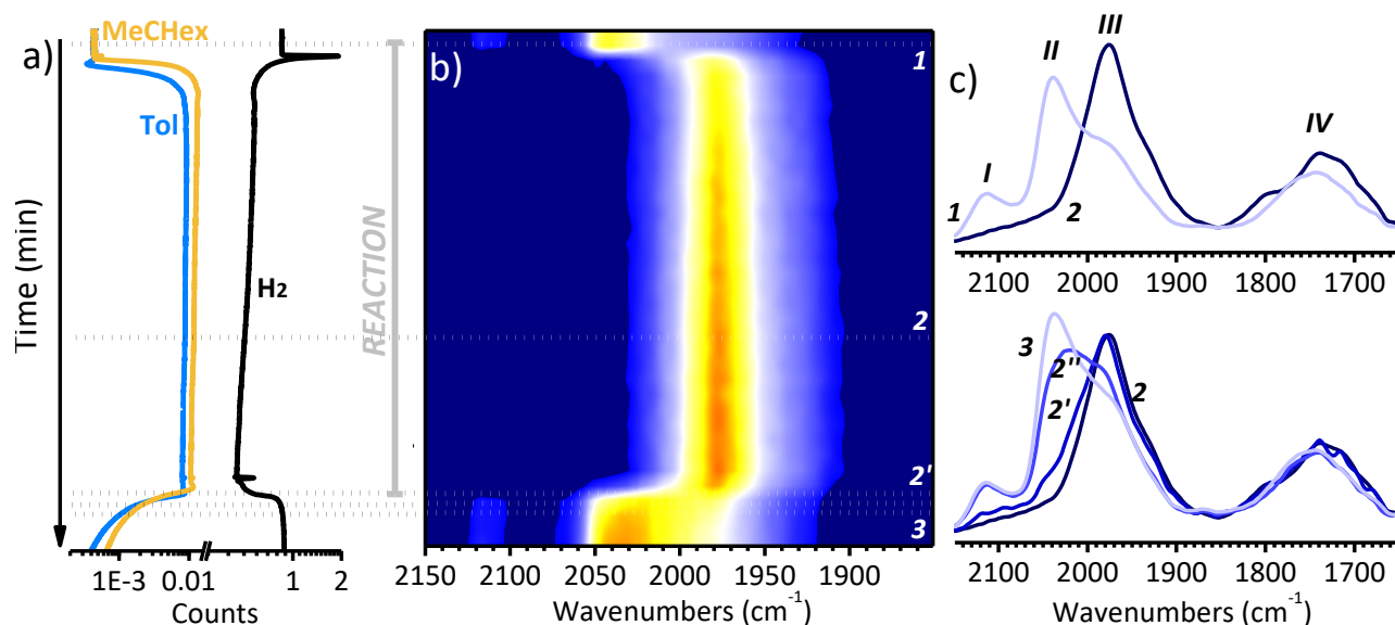
Figure 8. Part a): Evolution of the signals corresponding to \text{H}_2 ( m/Z=2 ), toluene ( m/Z=91 ) and methylcyclohexane ( m/Z=98 ), as detected by the mass spectrometer placed at the outlet of the reaction cell. Part b): 2D map showing the evolution of the DRIFT spectra as a function of time for the Pt/ \text{Al}_2\text{O}_3 catalyst during hydrogenation of toluene to methylcyclohexane at 120 °C. The reduction step preceding the reaction was accomplished in the presence of 10 mol% \text{H}_2 in He. The intensity increases from blue to red. Part c): FT-IR spectra selected at specific times as indicated in the 2D map shown in part b). The spectra are shown after subtraction of the spectrum of the catalyst before reduction, in the 2150-1850 \text{cm}^{-1} range.
