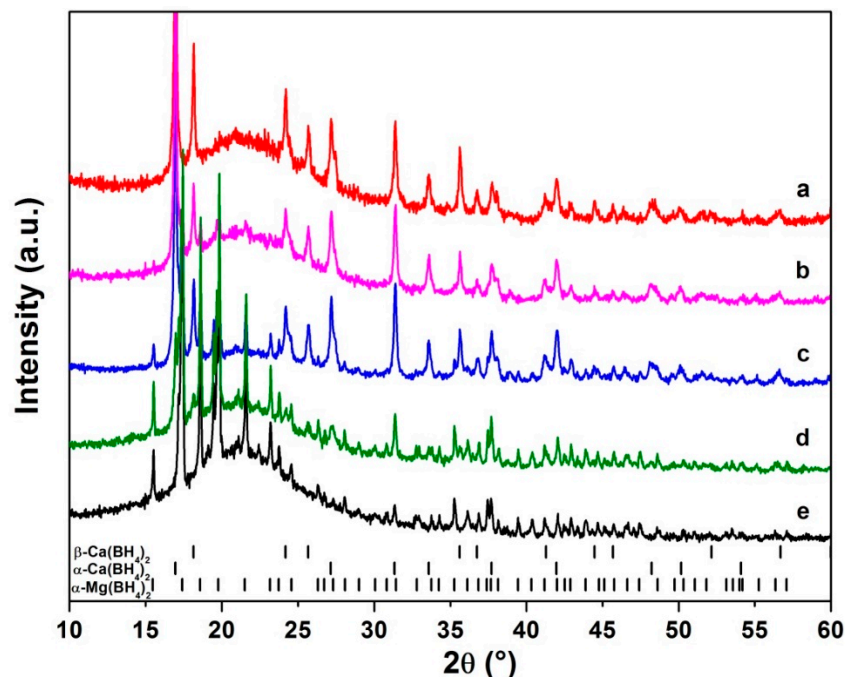
Figure 1. Powder X-ray diffraction (PXD) patterns of (a) \text{Ca}(\text{BH}_4)_2 , (b) 1\text{Mg}(\text{BH}_4)_2: 2\text{Ca}(\text{BH}_4)_2 , (c) 1\text{Mg}(\text{BH}_4)_2: 1\text{Ca}(\text{BH}_4)_2 , (d) 2\text{Mg}(\text{BH}_4)_2: 1\text{Ca}(\text{BH}_4)_2 , and (e) \text{Mg}(\text{BH}_4)_2 after ball milling.
