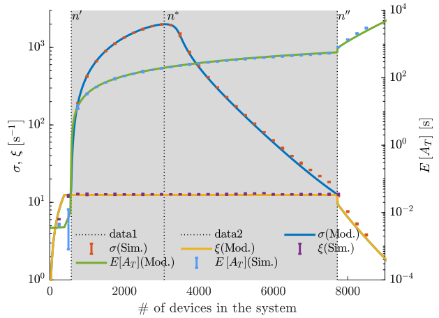
Figure 6: Model validation for a cell with 150 Mb/s capacity and p_a = 1.0 . Left scale for \sigma and \xi , right scale for access delay.
