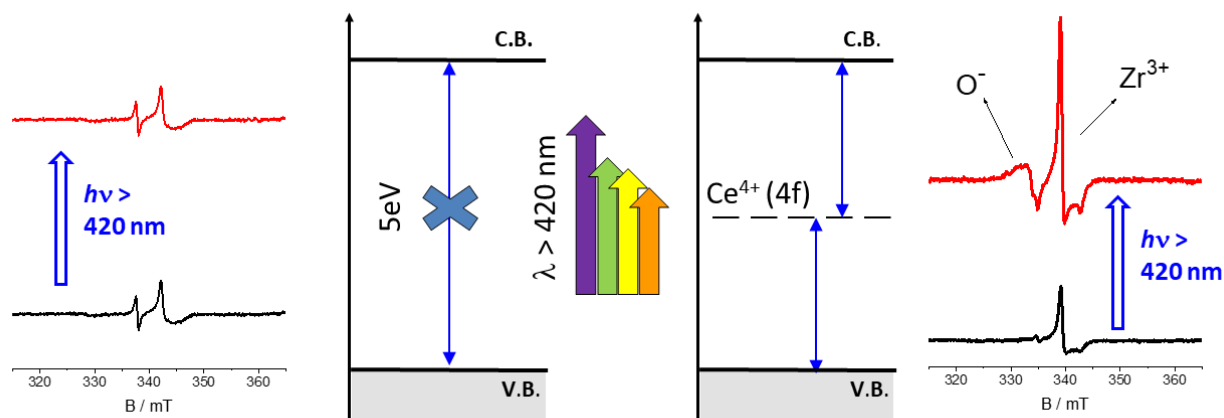
Figure 4. Effect of irradiation with polychromatic visible light having \lambda > 420 nm of pristine \text{ZrO}_2 (left) and \text{Ce-ZrO}_2 (right). The set of arrows in the figure compares the energy of the photons used in irradiation with the band gap of the systems.
