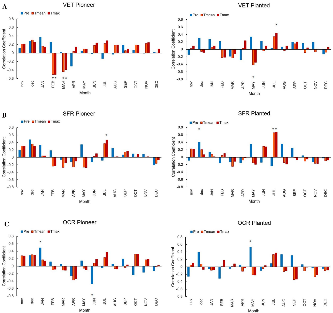
Fig. 7 Pearson's climate correlation between standardized IADFs chronologies and total monthly precipitation (Pre; blue) (Tmean; orange) and maximum (Tmax; red) monthly air temperatures
