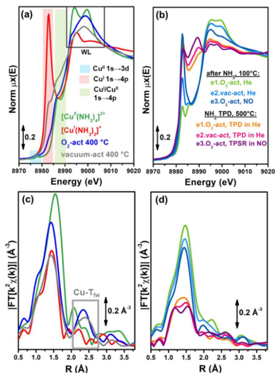
Figure 2. (a) Selected Cu K-edge XANES spectra of model Cu-species or catalyst states, including the [Cu II (NH 3 ) 4 ] 2+ and the [Cu I (NH 3 ) 2 ] + complexes and the O 2 -activated and vacuum -activated state of the Cu-CHA catalyst. The characteristic XANES fingerprints of Cu I and Cu II species are highlighted by coloured rectangles and summarized in Section 2.2.3. (b) XANES spectra of Cu-CHA at key stages during experiments e1-e3. (c, d) As parts (a) and (b), respectively, but reporting the corresponding the k 2 -weighted phase-uncorrected FT-EXAFS spectra, using the same colour code. The grey box in part (c) highlights the R-space region characteristic of Al/Si atoms (T fw ) scattering contributions.
