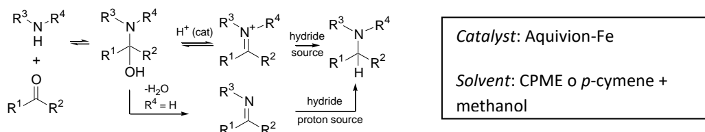
Figure 1: Reaction mechanism.
