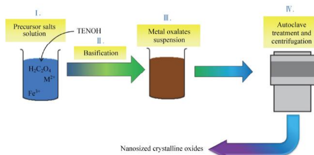
Figure 1: Synthesis scheme of transition metal ferrites [2].
