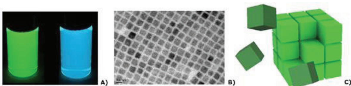
Figure 1: A) Bright emitting 11 nm (green) and 6 nm (blue) CsPbBr 3 nanocrystals dispersed in hexane; B) TEM image of CsPbBr 3 nanocrystals; C) Rendering of a possible self-assembled structure;
