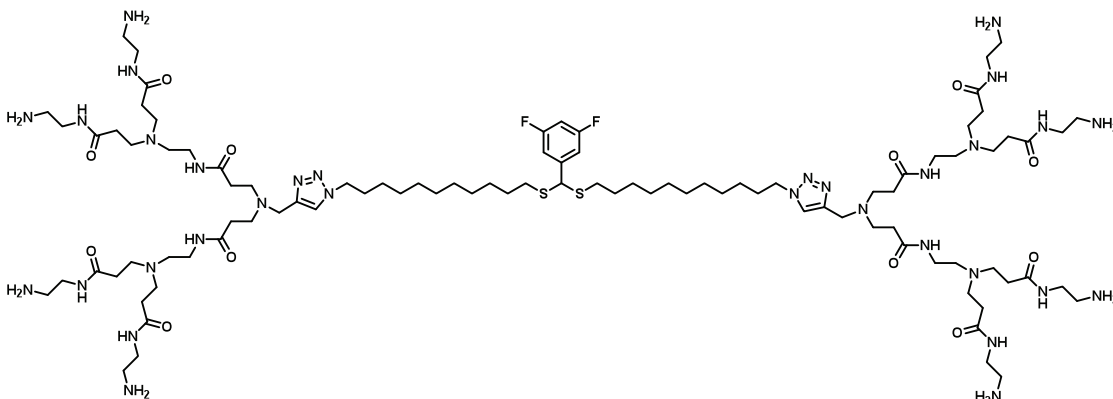
Figure 1 : Structure of Bola4A dendrimer reported in this work
