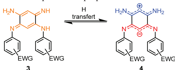
Figure 1: canonical/zwitterionic equilibrium of N,N' -disubstituted BQDI
