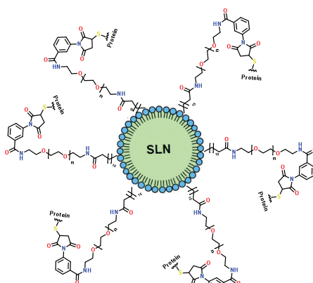
Figure 1 : Scheme of functionalized SLN
