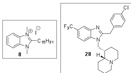
Figure 1: Chemical structure of the best-performing benzimidazole derivatives studied.
