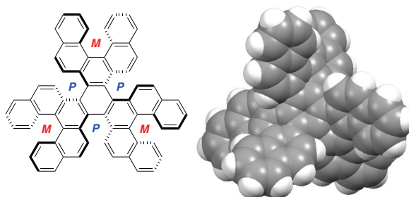
Figure 1 : D 3 -symmetric propeller-shaped nanographene 1 embedding six enantiomerically stable [5]helicenes
