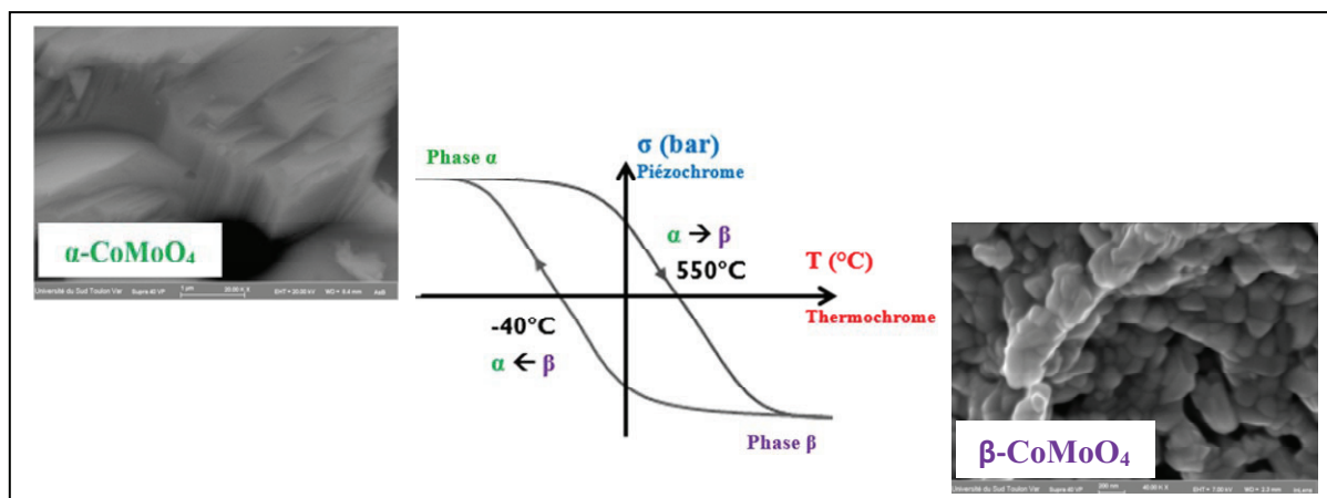
Figure 1. Phase transition of \text{CoMoO}_4 .
