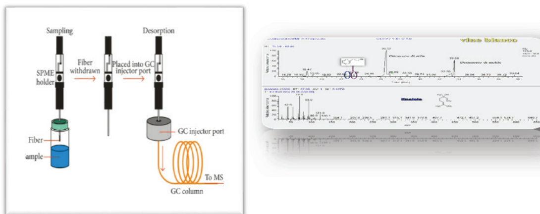
Figure 1 : FIG. 1: Solid phase microextraction and GCMS analysis
