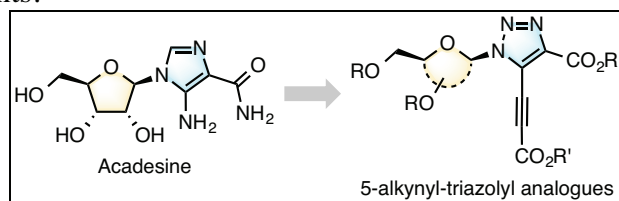
Figure 1 : From acadra to 3000-fold more potent analogues against MDS.
