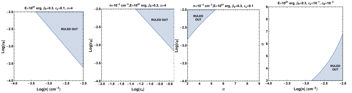
Figure 5. Allowed (white) and ruled out (shaded) parameter space of the KN afterglow of GW 170817 based on the fact that no re-brightening of the X-ray or radio emission was detected at \sim 2 yrs after the merger (Fig. 1). Two parameters are varied in each plot while the rest are kept fixed to values indicated in the plot title. The radio data set drives our conclusions and disfavors shallow stratification indexes \alpha \leq 6 . Future observations will further constrain the parameter space of the KN afterglow.
