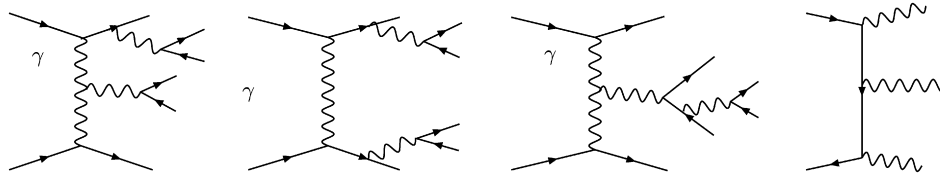
Fig. 2. Non-fusion and non-doubly resonant two vector boson production. Three vector boson production.
