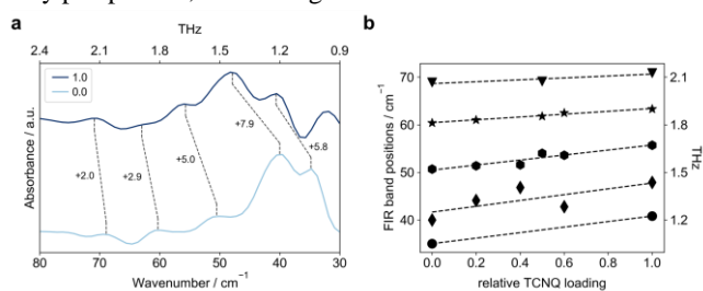
Figure 4. (a) Low frequency FIR spectra of \text{Cu}_3\text{BTC}_2 (light blue) and 1.0\text{TCNQ}@ \text{Cu}_3\text{BTC}_2 (dark blue). The spectra are normalized, and a vertical offset is applied for clarity. (b) Shift of FIR band positions with TCNQ loading. All corresponding FIR spectra are provided in the SI.
