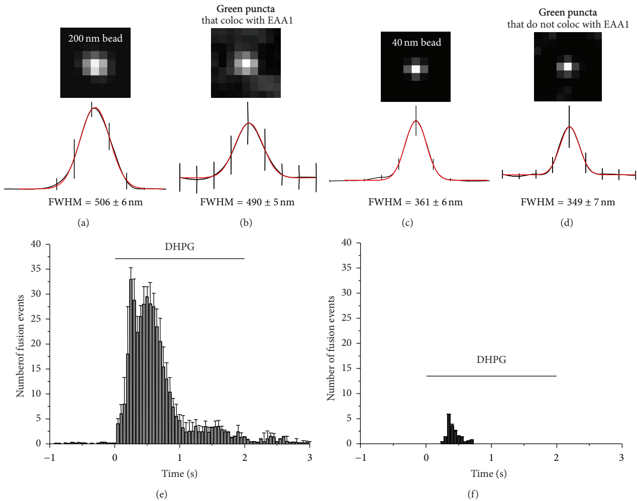
FIGURE 2: Analysis of VGLUT1-pHluorin vesicles that colocalize with markers of early or recycling endosomes. (a)–(d) Estimation of the size of vesicles expressing VGLUT1-pHluorin. Analysis of individual vesicle was performed in confocal images of VGLUT1-pHluorin-expressing astrocytes by plotting fluorescence intensity of pHluorin spots against distance from the centre of the spot (black curve \pm SD). Such an analysis provided an estimation of the average fluorescence profile otherwise called “radial sweep” [23]. The fluorescence intensity values obtained from the radial sweep were well fitted by a one-dimensional Gaussian function (red curve). Such a curve represents the average radial sweep value obtained from 20 vesicles. Note that the half maximum value of pHluorin-expressing vesicle positive for EAA1 ((b), marker of early endosomes, 490 \pm 5 nm) is similar to that of 200 nm fluorescent beads ((a), 506 \pm 6 nm) and the half maximum value of pHluorin-expressing vesicle that do not express EAA1 ((d), 349 \pm 7 nm) is similar to that of 40 nm fluorescent beads ((c), 361 \pm 6 nm). (e), (f) Temporal distribution of VGLUT1-pHluorin and Alexa-Tf 568 fusion events evoked by DHPG application. (e) Each individual histogram represents the number (mean \pm SD) of fusion events detected from VGLUT1-pHluorin vesicles in a 50 ms-long frame ( n = 5 cells). (f) Fusion events (mean \pm SD) detected from VGLUT1-pHluorin and Alexa-Tf568 double positive vesicles in the same cells as in (e). Each histogram represents the number of fusion events detected in a 50 ms-long frame ( n = 5 cells).
