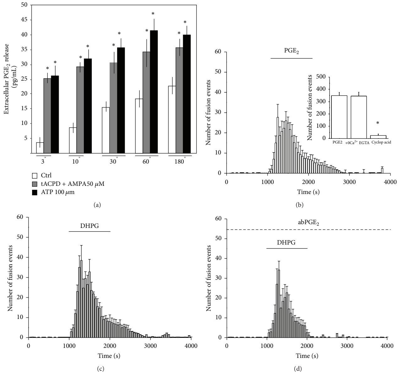
FIGURE 5: Extracellular PGE 2 : accumulation in response to various stimuli and effects on exocytosis of glutamatergic vesicles. (a). Extracellular accumulation of PGE 2 (expressed as pg/mL) in response to 3 min stimulation with either t-ACPD+ AMPA (each at 50 μM) or ATP (100 μM). Each point represents the average ± SEM of two experiments in triplicate with each stimulus. (b) Temporal distribution of fusion events evoked by PGE 2 (50 μM). Inset histograms represent the total number of fusion events evoked by PGE 2 (349 ± 26) in the presence of 0 mM Ca 2+ and 5 mM of EGTA (345 ± 32) or cyclopiazonic acid (CPA, 10 μM, 25 ± 12). (c) Temporal distribution of fusion events evoked by DHPG (100 μM). (d) Inhibitory effect of AbPGE 2 (buffering capacity >1000 pg/mL PGE 2 ) on exocytosis of glutamatergic vesicles evoked by DHPG (100 μM). Histograms represent temporal distribution of fusion events evoked by DHPG in the presence of AbPGE 2 . Statistical significance was calculated using t -test (* P < 0.05).
