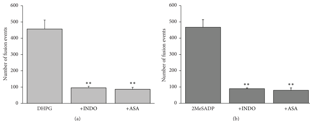
FIGURE 4: COX blockers strongly inhibit the exocytosis of glutamate evoked by activation of group I mGluR and of purinergic P2Y 1 receptor. (a), (b) Quantitative histograms represent the total number of fusion events evoked by either DHPG (100 μM, 456.7 ± 54.8) or 2MeSADP (20 μM, 467.6 ± 46.8) in the presence of COX blockers, INDO (1 μM; 94.9 ± 9.6, 88.8 ± 5.4, resp.) or ASA (10 μM, 86.4 ± 11.7, 79.5 ± 14.4, resp.). Data are ± SEM of 4 cells. Statistical significance of inhibition with receptor antagonists was calculated using t -test (** P < 0.01).
