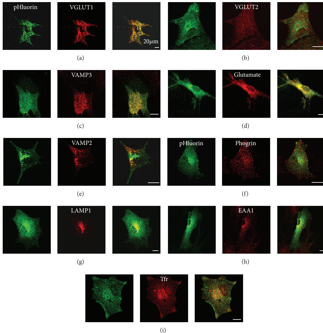
FIGURE 1: VGLUT1-pHluorin is mainly expressed on a specific population of glutamatergic synaptic like microvesicles. In the figure the left panels (in green) show astrocytes transfected with VGLUT1-pHluorin construct revealed by rabbit antibody against GFP. The middle panels (in red) show the markers of the intracellular secretory organelles, revealed by mouse antibodies against specific markers of ((a)–(e)) synaptic like microvesicles ((a) VGLUT1, (b) VGLUT2, (c) VAMP3, (d) glutamate, (e) VAMP2), of (f) dense core granules (phogrin), of (g) late endosomes, multivesicular bodies and lysosomes (LAMP1), of (h) early endosomes (EAA1), and of (i) recycling endosomes (transferrin receptor, Tfr). The right panels show the merged images. Bars: 20 \mu\text{m} .
