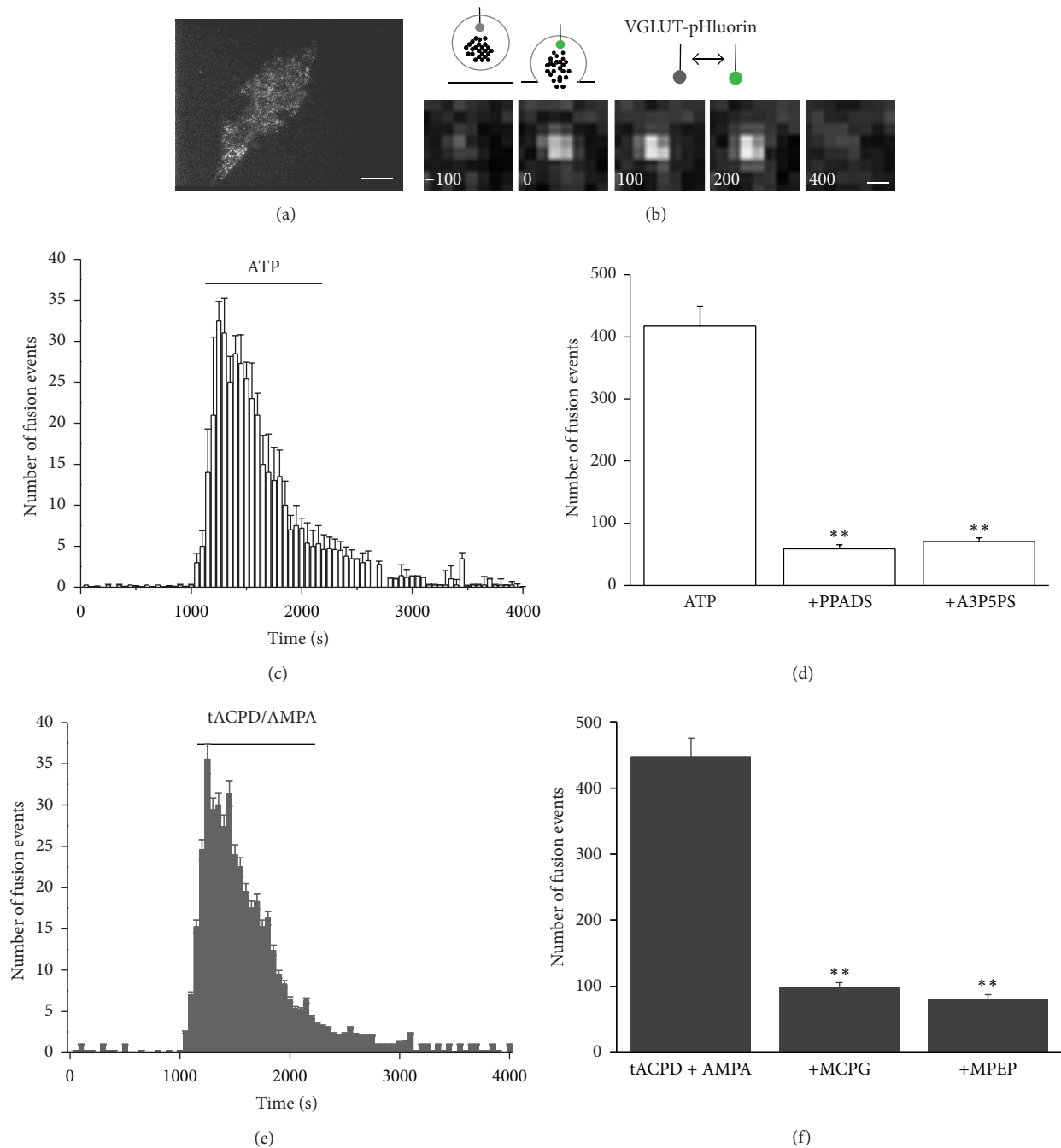
FIGURE 3: Pharmacological characterization of the receptor subtypes mediating exocytosis of VGLUT1-pHluorin positive vesicles in response to ATP and glutamate agonists. (a) TIRF image showing an astrocyte transfected with VGLUT1-pHluorin. Bar 20 nm. (b) Stereotyped sequence of pHluorin fluorescence before and during exocytosis of a VGLUT1-pHluorin positive vesicle. The sequential gray scale micrographs represent the fate of pHluorin before (-100 ms) and during (100, 200, 400 ms) the fusion event. Bars: 380 nm. The scheme shows the behaviour of pHluorin before and after fusion event. Note that the color code for the pHluorin fluorescence signal is gray when the signal is off and green when it is on. (c), (d) P2Y 1 receptors mediate the ATP-evoked exocytosis. (c) Temporal distribution of fusion events evoked by ATP (100 \mu M). (d) Histograms represent the total number of fusion events evoked by ATP (417.14 \pm 32.4) that is strongly inhibited in the presence of the P2 purine antagonists PPADS (100 \mu M, 58.6 \pm 7) as well as of the P2Y 1 -selective compound, A3P5PS (100 \mu M, 70.2 \pm 5.8). Data are \pm SEM of 4 cells. (e), (f) mGluR5 mediates the response to t-ACPD, in the presence of AMPA. (e) Temporal distribution of fusion events evoked by 50 \mu M t-ACPD + 50 \mu M AMPA. (f) Histograms represent the total number of fusion events evoked by t-ACPD + AMPA (447.1 \pm 28.7) that is strongly inhibited in the presence of the mGluR antagonists, including the subtype-nonselective MCPG (500 \mu M, 98.3 \pm 7.4) and the mGluR5-selective MPEP (200 nM, 80.1 \pm 7). Data are \pm SEM of 4 cells. Statistical significance of inhibition with receptor antagonists was calculated using t -test (** P < 0.01).
