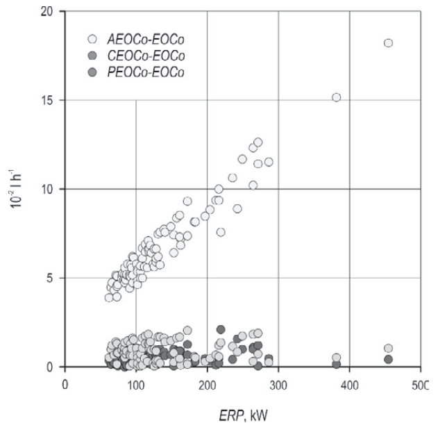
Fig. 7 Plots of absolute differences between manufacturers’ engine oil consumption of 133 examined machines EOCo and predicted engine oil consumption of: 1) this study ( PEOCo , dark gray); 2) Calcante et al. ( CEOCo , medium grey); 3) ASABE Standard D497.7 ( AEOCo , light grey)
