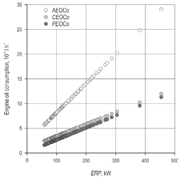
Fig. 6 Different predicted engine oil consumptions ( 10^{-2} \text{ l h}^{-1} ): this study ( PEOCo , dark grey), ASABE Standard D497.7 ( AEOCo , light grey) and Calcante et al. (2017) ( CEOCo , medium grey), as a function of engine rated power ERP (kW)
