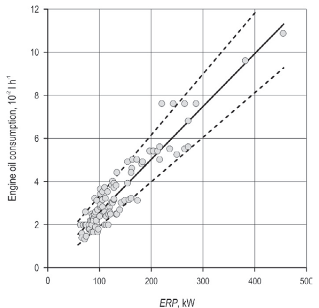
Fig. 2 Plot of engine oil consumption every 100 hours of machine work (10 -2 l h -1 ) as a function of engine rated power ERP (kW), regression line PEOCO and 95% confidence interval
