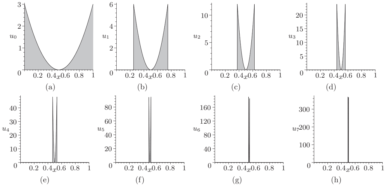
FIGURE 1: First 7 iterations of operator T^* defined in (11) for the only map w(x) = \frac{1}{2}x + \frac{1}{4} together with the only greyscale map \phi(y) = 2y starting from u_0(x) = 12(x - \frac{1}{2})^2 .
