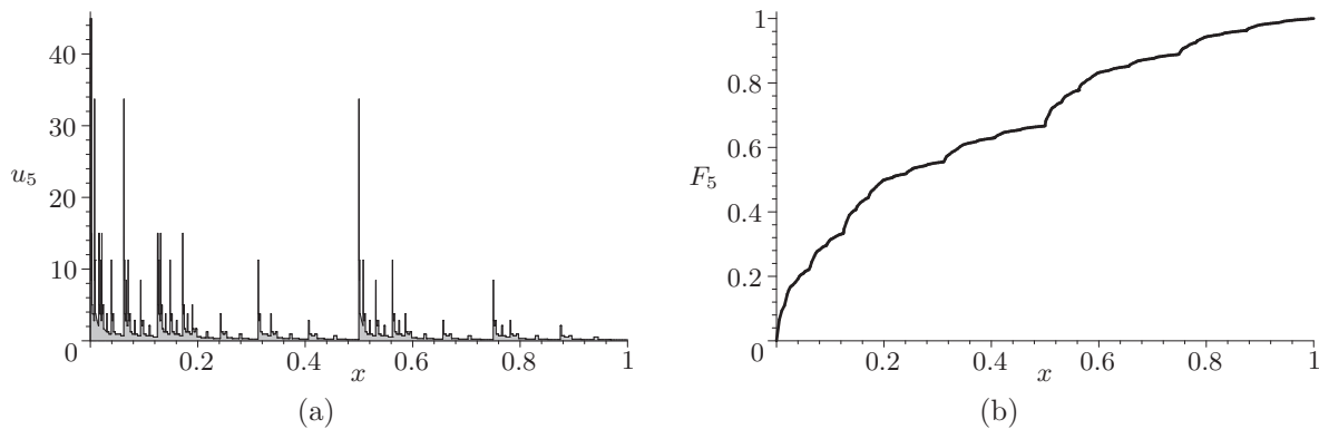
FIGURE 8: a) 5 th iteration of operator T_3^* defined in (16) for the maps w_1(x) = \frac{1}{8}x , w_2(x) = \frac{3}{8}x + \frac{1}{8} and w_3(x) = \frac{1}{2}x + \frac{1}{2} together with greyscale maps \phi_1(y) = \frac{8}{3}y , \phi_2(y) = \frac{8}{9}y and \phi_3(y) = \frac{2}{3}y starting from u_0(x) \equiv 1 , b) its associated cumulative distribution function.
