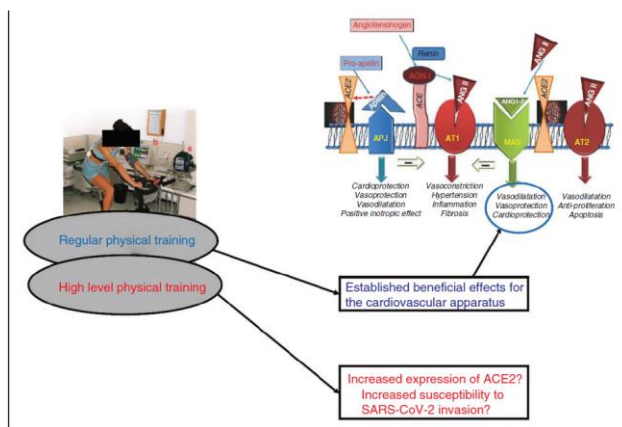
Figure 1. Simplified diagram showing the connection between physical training and the renin–angiotensin system. Top insert: schematic model of the angiotensin-converting enzyme (ACE) and ACE2 interactions at the cell membrane level. These two enzymes are aminopeptidases that remove amino acids from precursors to obtain ligands (i.e. angiotensin ANG II and ANG 1-7), which will bind to receptors (ANG II receptor (AT) ANG 1-7 receptor (MAS), respectively) obtaining specific effects on the cardiovascular system. Physical training can affect ACE2 expression, while coronavirus can interfere with ACE2 activity. Also apelin and its G-protein coupled receptor (APJ) are linked to ACE2 and apelin overexpression has been linked to physical training.
