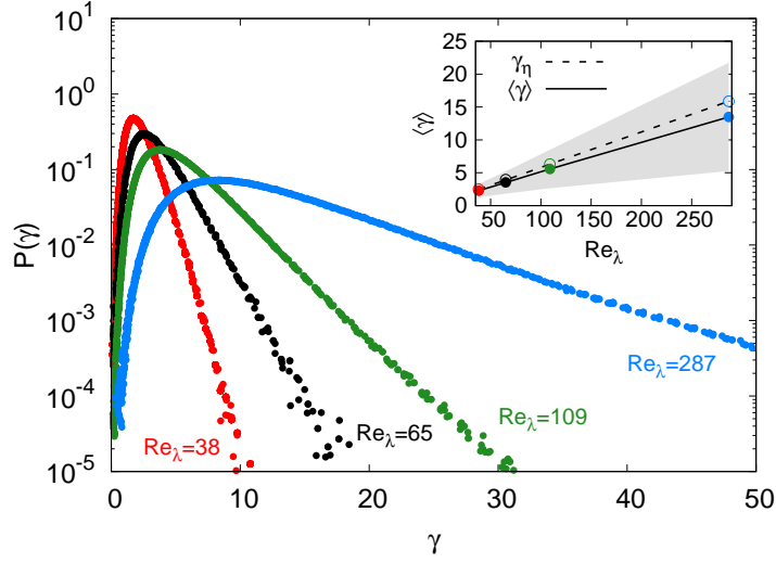
FIG. 2. (color online) Probability density function of shear rate \gamma = (2S^2)^{1/2} for different Re_\lambda . Inset: mean shear rate \langle \gamma \rangle (filled circles with solid line) and its root mean square (area in gray) compared with the dimensional estimation \gamma_\eta = \tau_\eta^{-1} (empty circles with dashed line), due to the Jensen inequality \langle \gamma \rangle < \gamma_\eta .
