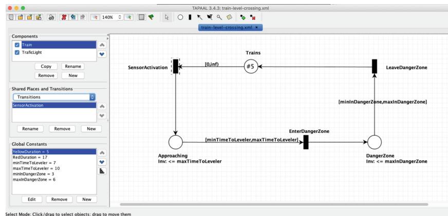
Fig. 3. Screenshot of TAPAAL GUI
