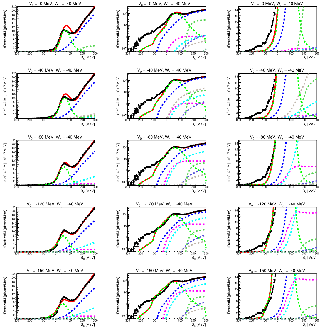
Fig. B.1. Detailed comparison between the data and the template t with various V_0 values. The imaginary part is fixed to the optimum value W_0 = -40 MeV. The title of each plot shows the V_0 values. The green dotted lines show the theoretical calculations for the K^-p quasi-elastic process obtained by the Green's function method. The other colored dotted lines show the calculated spectral shapes for the background processes (see Fig. 11). The total fit results are displayed by red lines. The left and middle columns show the same spectra with linear and semi-log scales, respectively, and the right column shows the magnified view for a small cross section region.
