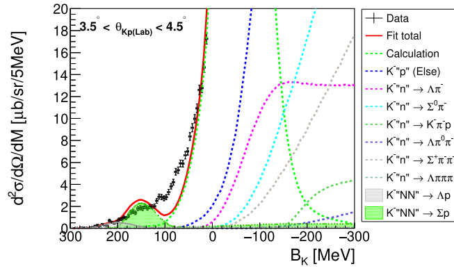
Fig. D.2. (a) The magnified view of the small cross section of the template fit result by adding the one-step two-nucleon absorption processes. The components of K^-NN \rightarrow \Lambda p and K^-NN \rightarrow \Sigma p are displayed by gray and green hatched spectra, respectively. The green dotted line shows the calculated spectrum with the optical potential of (V_0, W_0) = (-80, -40) MeV. The other color assignments are the same as in Fig. 11.
