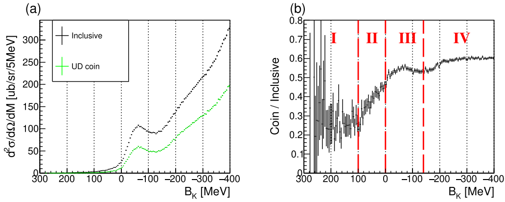
Fig. 18. (a) Comparison between the inclusive and coincidence spectra shown by black and green points, respectively. (b) Coincidence probability spectrum calculated by dividing the coincidence spectrum by the inclusive spectrum.
