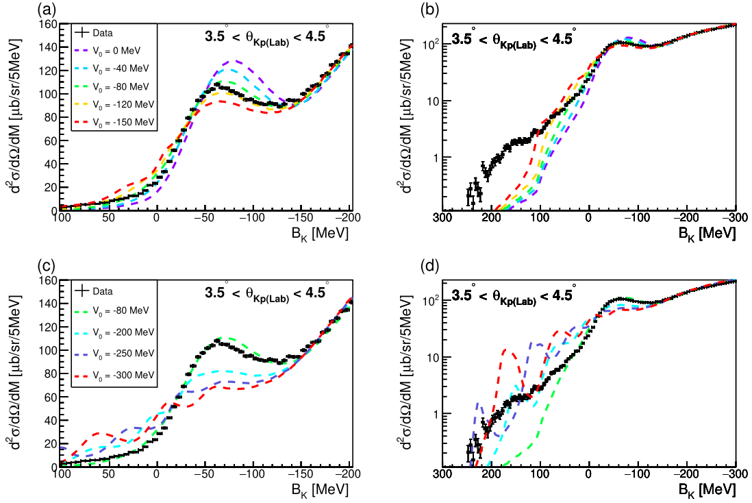
Fig. 12. Comparison between the measured spectrum and template with different optical potentials. The black points with error bars display the measured spectrum. The dashed lines in different colors show the template results using different potential depths of the real part ( V_0 ). The imaginary part is fixed at the optimum value of W_0 = -40 MeV. The comparisons with the real part potentials of V_0 = (0, -40, -80, -120, -150) MeV and V_0 = (-80, -200, -250, -300) MeV are shown in (a, b) and (c, d), respectively. The spectra with linear and semi-log scale are shown in (a, c) and (b, d), respectively.
