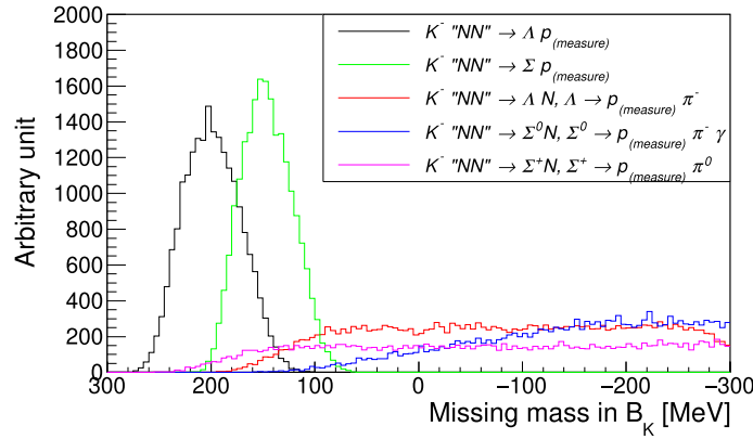
Fig. D.1. Simulated missing-mass spectra of the ^{12}\text{C}(K^-, p) reaction for one-step two-nucleon absorption processes plotted in the scale of B_K ; p_{(measured)} is the proton measured by our spectrometer.
