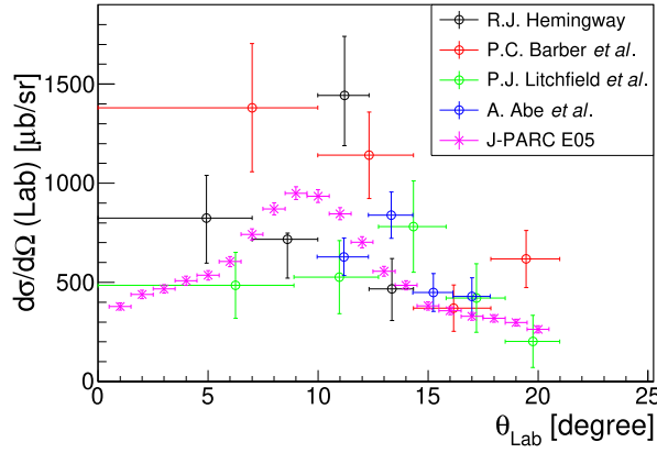
Fig. 10. Compilation of differential cross sections of the K^-p elastic scattering at p_{K^-} = 1.8 \text{ GeV}/c . Our results are shown by the magenta points with statistical errors. The previous data [44–47] are also displayed in different colors.
