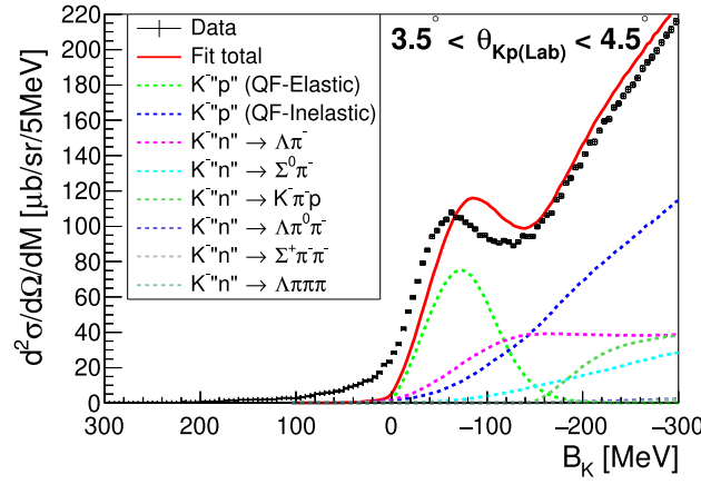
Fig. 11. Double differential ^{12}\text{C}(K^-, p) cross section as a function of K^- binding energy, B_K . The forward scattering angle range of 3.5^\circ < \theta_{Kp(\text{Lab})} < 4.5^\circ is selected. The black points with statistical error bars show the measured double differential cross section, and different colors show the template- t results. The green dotted line shows the K^-+p \rightarrow K^-p quasi-elastic component, calculated by the Green's function method. In this t, we do not include secondary interactions inside the target nucleus. See the details in the text.
