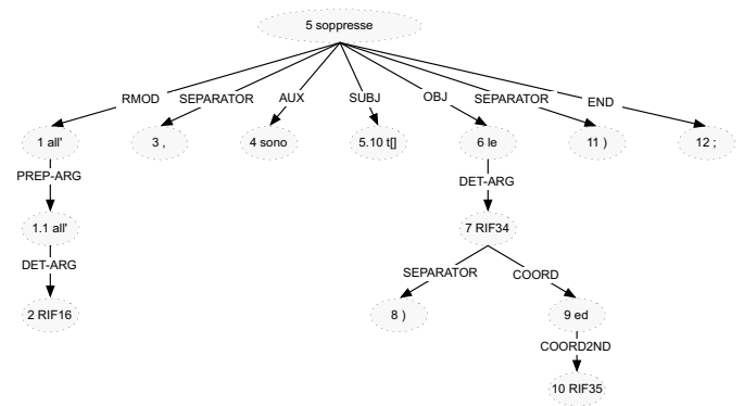
Figure 6: Parse tree of coordinated repeals.
