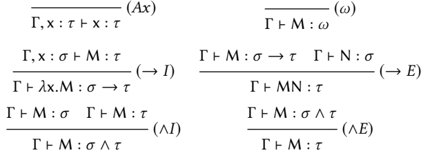
Figure 7. Typing rules for intersection types.
