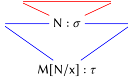
Figure 2. Derivation of M[N/x] : \tau when x occurs exactly once in M .
