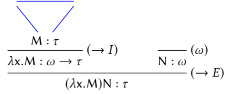
Figure 5. Derivation of (\lambda x.M)N : \tau when x does not occur in M .
