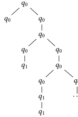
Figure 12. A run tree of \mathcal{B} for the tree in Figure 11.
