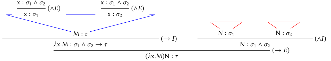
Figure 6. Derivation of (\lambda x.M)N : \tau when x occurs twice in M .
