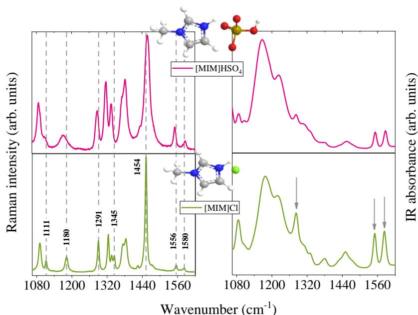
Figure 3: Comparison between UVRR spectra excited at 250 nm (panel on the left) and IR absorption spectra (panel on the right) of neat [MIM]HSO 4 and neat [MIM]Cl.
