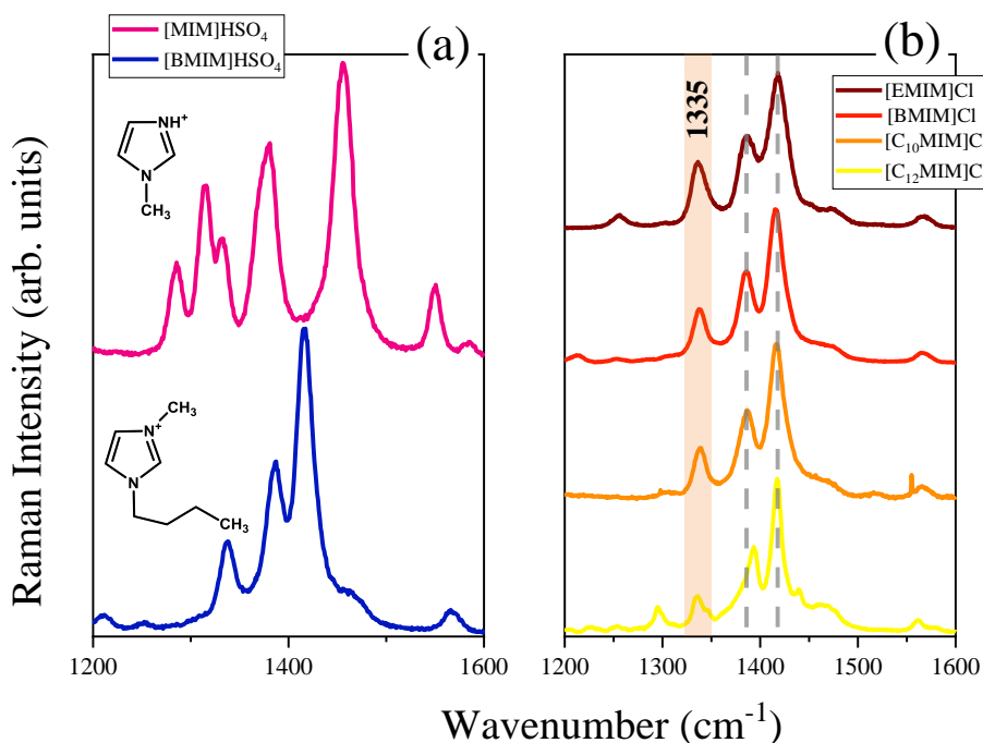
Figure 4: Comparison between the UVRR spectra (excited at 250 nm) of (a) [MIM]HSO 4 and [BMIM]HSO 4 and of (b) [EMIM]Cl, [BMIM]Cl, [C 10 MIM]Cl and [C 12 MIM]Cl.
