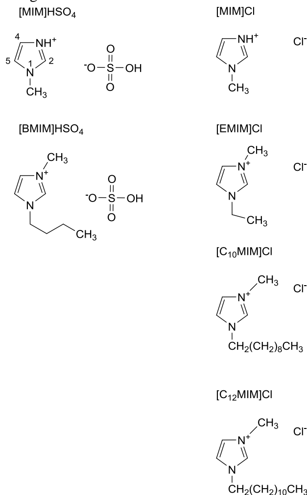
Figure 1: Chemical structure of ionic liquids investigated in this work.
