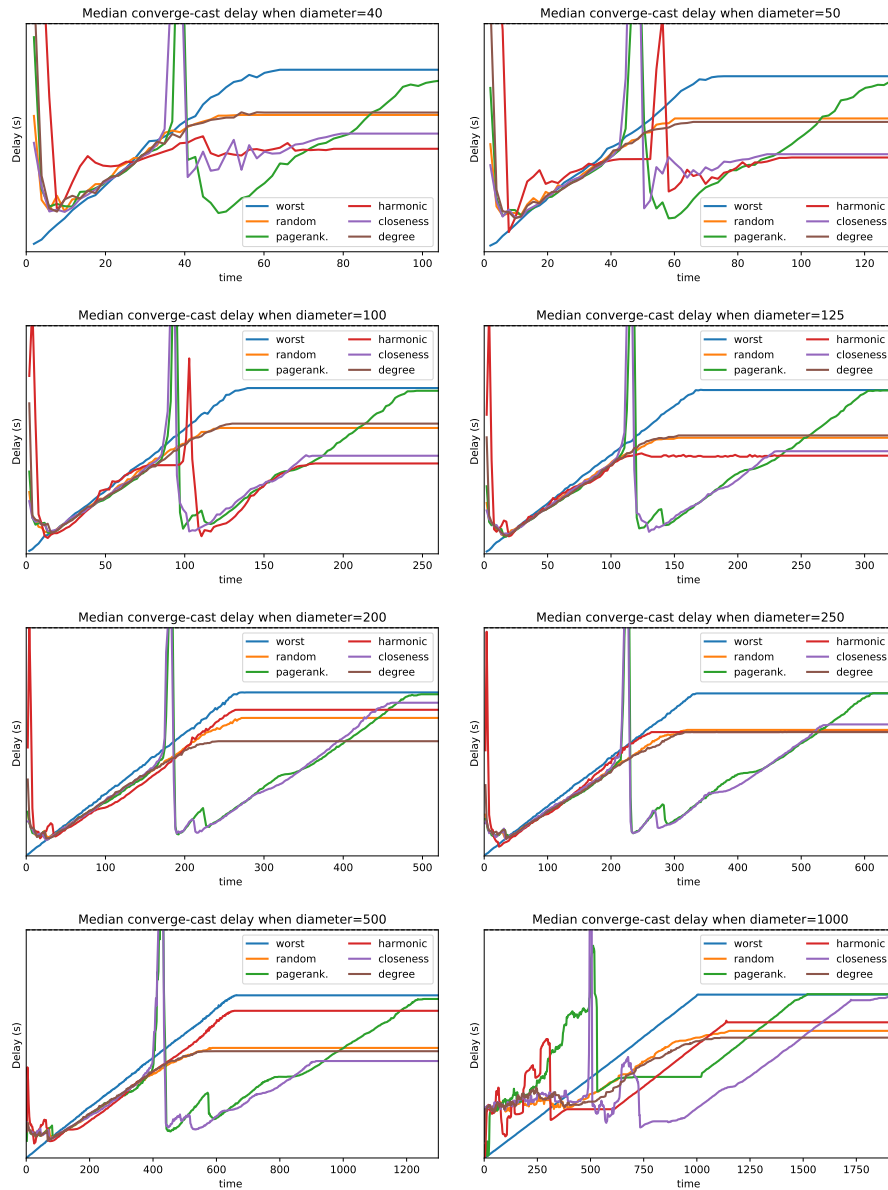
Figure 15: Median delay for converge-cast with different algorithms for leader election for different network shapes, ranging from a 40 \times 25 (top left) to a 1000 \times 1 grid (bottom right). Pagerank performs badly across the board, with a performance comparable to the worst case. Degree centrality's results show a behaviour only slightly improving over a random selection. Harmonic centrality outperforms every other algorithm in grids up to 125 \times 8 , followed closely by closeness centrality. In the most extreme quasi-linear scenarios, degree centrality attains the best results.
