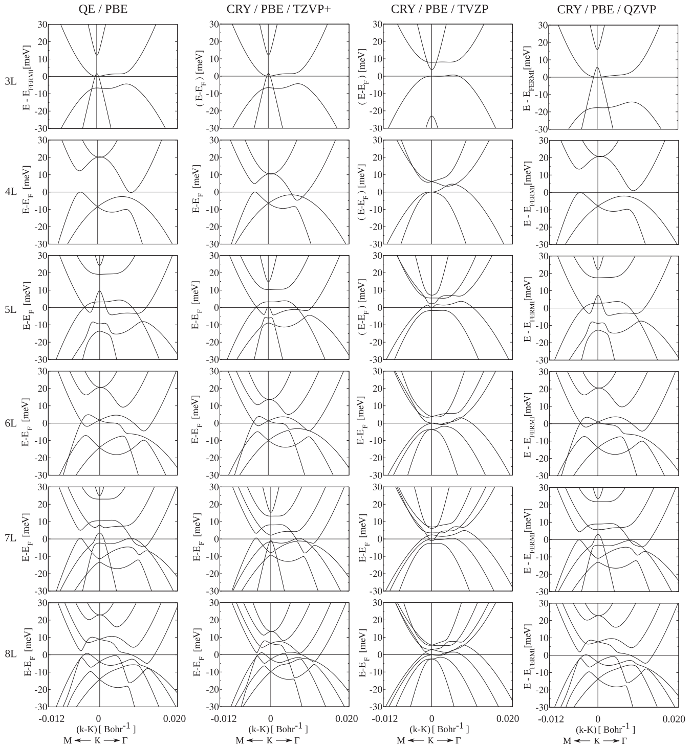
FIG. 3. PBE band structure of all studied multilayer systems with Bernal stacking. On the left are reported the calculations carried out with QE, while on the other columns the calculations made exploiting the CRYSTAL code, using different basis sets. From left to right we have the TVZP+ basis set, the standard TVZP basis set, and finally the QZVP basis set.
