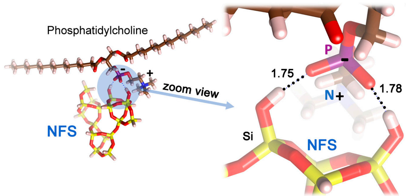
Fig. 6. A cluster model of nearly-free silanols (NFS) interacting with phosphatidylcholine, a building block of cell membranes, as predicted by the GFN-FF calculations. The H + O hydrogen bond distances between the NFS and the oxygens of the negatively charged phosphate group are in ångströms.
