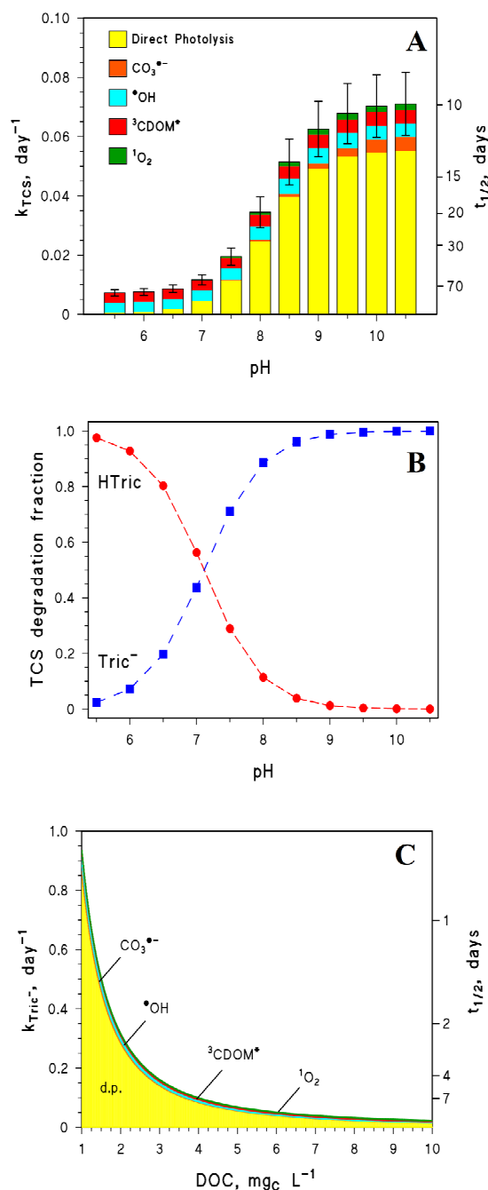
Figure 2. (A) Simulated pseudo-first order photodegradation rate constants of TCS (left Y-axis) and corresponding half-life times (fair-weather sunny days, right Y-axis), as a function of pH ( \text{DOC} = 5 \text{ mg}_C \text{L}^{-1} ). The role of the different photochemical processes is highlighted with different colors. (B) Trend with pH of the relative roles of \text{HTric} and \text{Tric}^- in TCS photodegradation ( \text{DOC} = 5 \text{ mg}_C \text{L}^{-1} ). (C) \text{Tric}^- photodegradation kinetics as a function of the water DOC (d.p. = direct photolysis). Other conditions: 10^{-4} \text{ mol L}^{-1} nitrate, 10^{-6} \text{ mol L}^{-1} nitrite, 10^{-3} \text{ mol L}^{-1} alkalinity, 5 m water depth. The error bounds in (A) are the sigma-level model uncertainties on the values of the overall pseudo-first order degradation rate constants of TCS.
