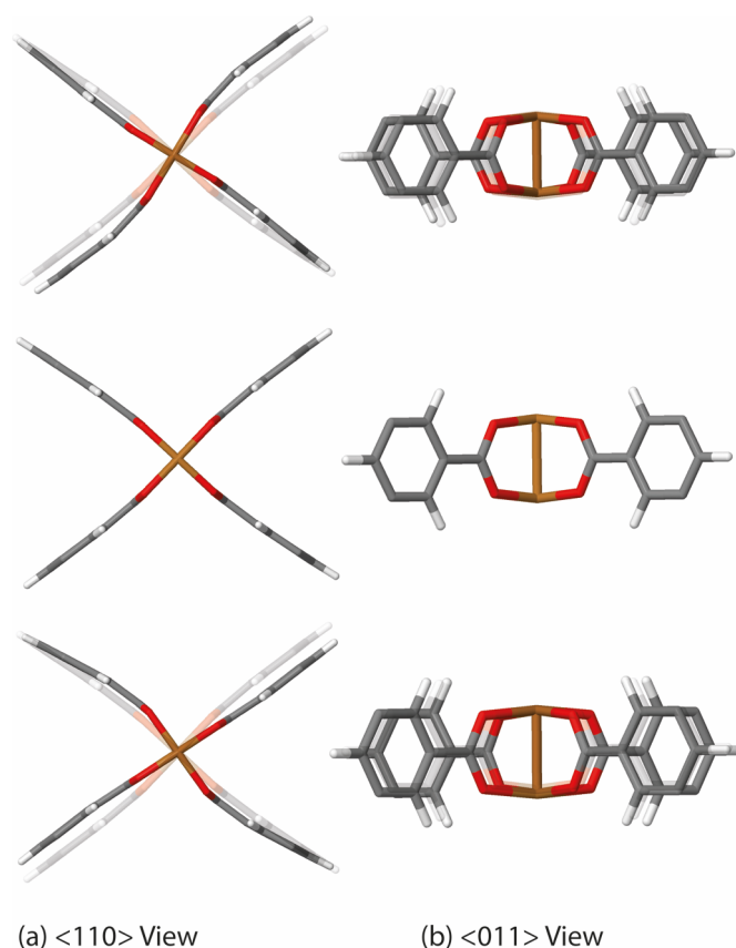
Fig. 4 Low energy collective vibration, located at 58\text{ cm}^{-1} (1.7 THz), viewed down the (a) \langle 110 \rangle and (b) \langle 011 \rangle directions, showing a rotor motion of the Cu-based paddle-wheel moiety. Videos of the motions are available in the ESI.
