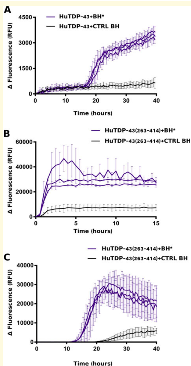
Figure 2 RT-QuIC analysis of BH samples. In brief, 20 \mu\text{L} of sonicated and diluted ( 10^{-3} ) BHs collected from three FTLTDP patients (BH*, purple lines) and one CTRL patient (CTRL BH, black line) were added to purified seed-free recombinant HuTDP-43 (1 mg/mL) (A) and HuTDP-43(263-414) (0.2 mg/mL) (B) and analysed by means of RT-QuIC. The reaction was exposed to 60 s of shaking and 60 s of rest. All positive BHs efficiently seeded the reaction, whereas the negative control BH at the same dilution ( 10^{-3} ) did not affect the aggregation kinetics of the reaction. (C) Optimized protocol for BH analysis using purified seed-free HuTDP-43(263-414) (0.05 mg/mL) as substrate with a different reaction buffer (no NaCl, Gdn-HCl added) and a modified protocol (shaking at 100 rpm for 15 s every 30 min at 40°C). ThT fluorescence intensity was plotted against time. Each graph has a specific range of ThT fluorescence values and duration of a given reaction. The experiment was performed in triplicate and each replica was performed three times. Curves represent means for all experimental replicates and bars indicate the standard deviations (SD).
