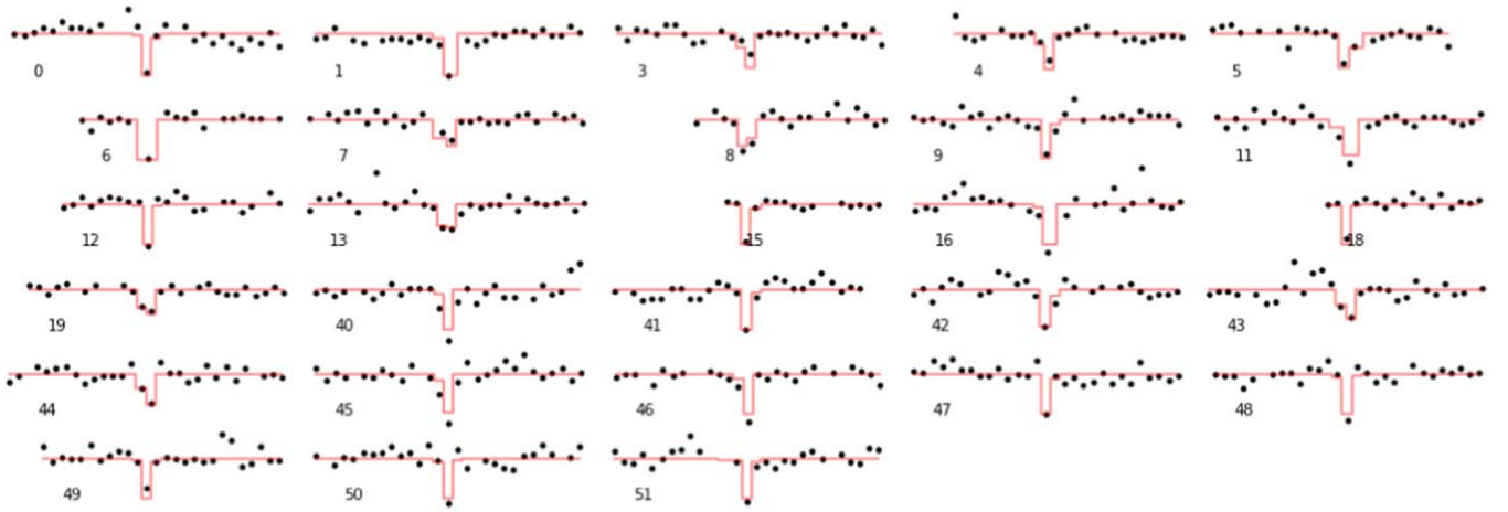
Figure B.4. Individual transits of K2-146 c fitted in the PyTTV transit parameter analysis. This figure uses the same notations as Figure B.3. The individual transit times are available as data behind the Figure.
