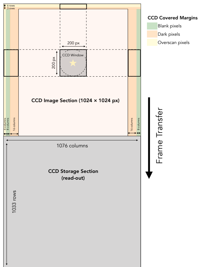
Fig. 8 Schematic view of the CCD elements.
