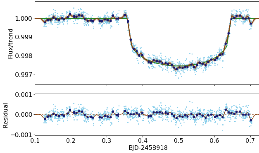
Fig. 15 Observed light curve of KELT-11 and model fit from pycheops. The measured fluxes (light blue points) are also shown binned in time (dark blue points). The transit model (green line, barely visible) is shown in the upper panel together with the several realisations of our complete model including stellar noise sampled from the PPD. The lower panel shows residuals from the transit model plus instrumental effects (blue points) together with the best-fit stellar noise model (brown line).
