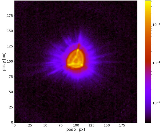
Fig. 13 CHEOPS has a de-focused PSF where 90 % of the total energy is inside a radius of 16 pixels. In this figure the PSF flux distribution in white light is shown as measured during the in-orbit commissioning.
