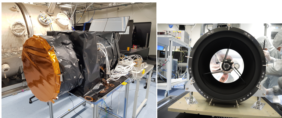
Fig. 6 Left: The CHEOPS payload fully assembled before delivery. Right: The telescope with mirrors installed and cover open before full OTA assembly.
