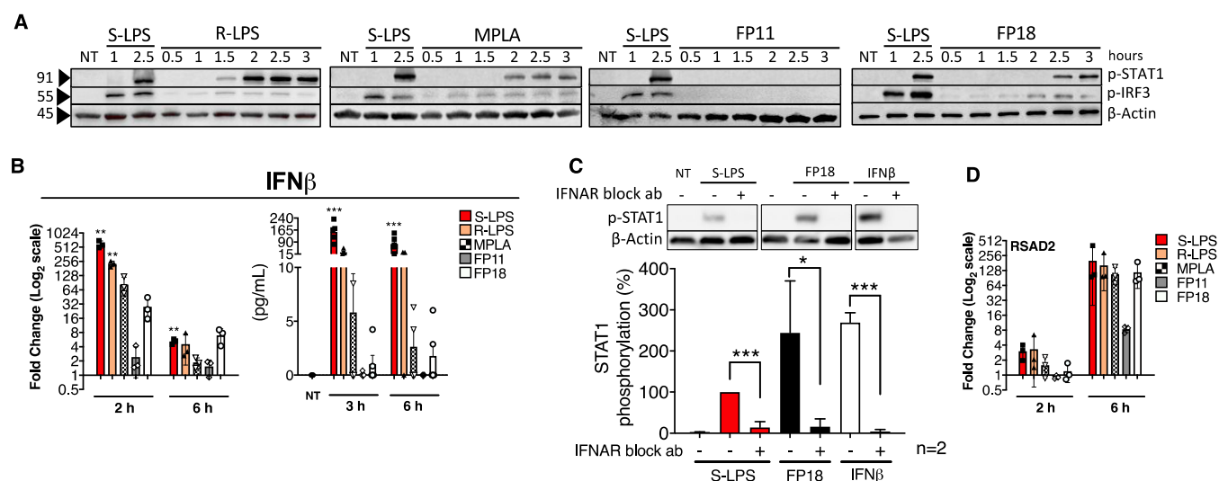
Figure 5. (A) Trehalose dimycolate (TDM) was treated with S-LPS (100 ng/mL), R-LPS (100 ng/mL), MPLA (1 \mu g/mL), FP11 (10 \mu M), FP18 (10 \mu M), or left untreated (NT) and collected after the indicated time. The levels of phospho-IRF3, phospho-STAT1, and actin were detected by immunoblotting. (B) TDM was treated as in panel A and collected after the indicated time. (Left) IFN \beta production is expressed as fold change compared to untreated cells. Error bars represent SD of the mean; n = 3 , where * p < 0.05 , ** p < 0.01 , and *** p < 0.001 . Statistical analysis is between treated vs untreated (Wilcoxon's test). (Right) IFN \beta release was quantified by ELISA. Error bars represent SD of the mean; n = 4 where * p < 0.05 ; ** p < 0.01 ; and *** p < 0.001 . Statistical analysis is between treated vs untreated (NT) (one-way ANOVA test). (C) TDM was pretreated with IFNAR2 neutralizing antibody (1 \mu g/mL) 1 h prior to exposure to the indicated stimulus. Cell lysates were collected after 3 h and p-STAT1 was measured via immunoblotting. Error bars represent SD of the mean; n = 2 where * p < 0.05 and *** p < 0.001 (one-way ANOVA test). (D) TDM was treated as in panel B and collected after the indicated time. RSAD2 expression is expressed as fold change compared to untreated cells. Error bars represent SD of the mean; n = 3 , where * p < 0.05 , ** p < 0.01 , and *** p < 0.001 . Statistical analysis is between treated vs untreated (Wilcoxon's test).
