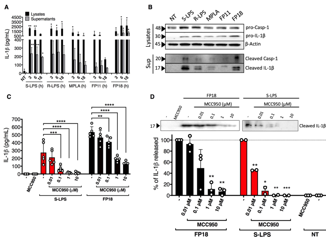
Figure 6. (A) TDM was treated with S-LPS (100 ng/mL), R-LPS (100 ng/mL), MPLA (1 μg/mL), FP11 (20 μM), FP18 (20 μM), or left untreated. IL-1β levels were measured in both cell lysates and supernatants by ELISA. Error bars represent SD of the mean; n = 3 where *p < 0.05 , **p < 0.01 , and ***p < 0.001 . Statistical analysis is between treated vs untreated (NT) (one-way ANOVA test). (B) TDM was treated as in panel A for 6 h. Levels of pro-casp-1/pro-IL-1β, and cleaved casp-1/cleaved-IL-1β were detected by immunoblot in cell lysates and supernatants, respectively. (C, D) TDM was pretreated for 1 h with an increasing concentration of MCC950 and then stimulated with S-LPS (100 ng/mL) or FP18 (20 μM) for 6 h. The effect of MCC950 on LPS- and FP18-triggered IL-1β secretion was evaluated by ELISA (C) and immunoblot (D). In (C), error bars represent SD of the mean; n = 5 where *p < 0.05 , **p < 0.01 , and ***p < 0.001 (one-way ANOVA test). In (D), the percentage of IL-1β release was normalized to stimulation with only S-LPS or only FP18, and error bars represent SD of the mean ( *p < 0.05 , **p < 0.01 , and ***p < 0.001 , Wilcoxon's test).
