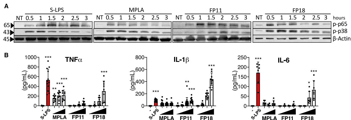
Figure 4. (A) TDP were treated with S-LPS (100 ng/mL), MPLA (1 \mu g/mL), FP11 (10 \mu M), FP18 (10 \mu M), or left untreated (NT) and collected after the indicated time. The levels of phospho-p65, phospho-p38, and actin were detected by immunoblotting. (B) In vitro cytokines released from TDP measured by enzyme-linked immunosorbent assay (ELISA). Cells were treated with S-LPS or with increasing concentrations of MPLA, FP11, and FP18 (0.1–1 to 10–25 \mu M) for 18 h. Error bars represent the SD of the mean. TNF \alpha ( n = 9 ), IL-1 \beta ( n = 9 ), and IL-6 ( n = 7 ), where * p < 0.05 , ** p < 0.01 , and *** p < 0.001 . Statistical analysis is between treated vs untreated (-) (one-way analysis of variance (ANOVA) test).
