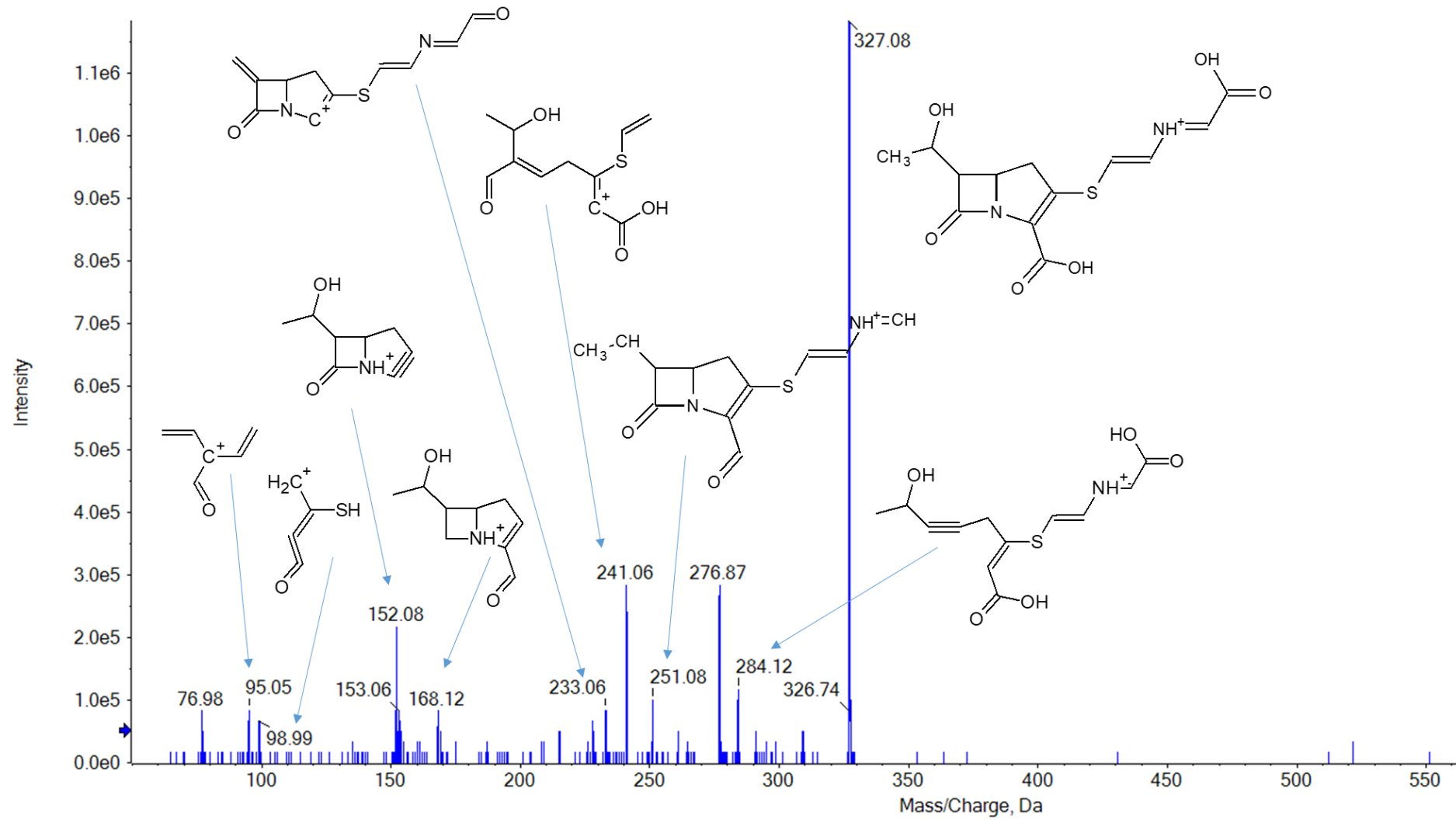
Figure S33. ESI (PI) MS/MS spectrum of IMI-P3.
