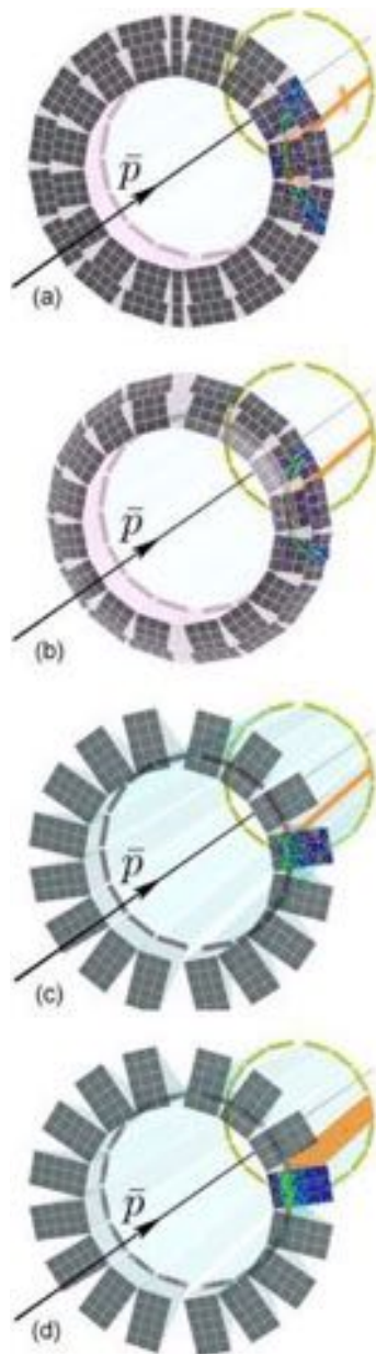
Figure 20. Geant simulation of the \bar{P} ANDA Barrel DIRC using different design options. An oil tank with a straight (a) or curved (b) imaging plane is shown at the top. Solid fused silica prisms are used as EV in the design on the bottom (c), (d). Narrow bars (a)–(c) or wide plates (d) are used as radiator. Cherenkov photon trajectories from a 3 GeV/c kaon are shown in orange. The colored histogram shows the accumulated hit pattern from 100 kaons of the same momentum. Reprinted from [43], Copyright (2014), with permission from Elsevier.
