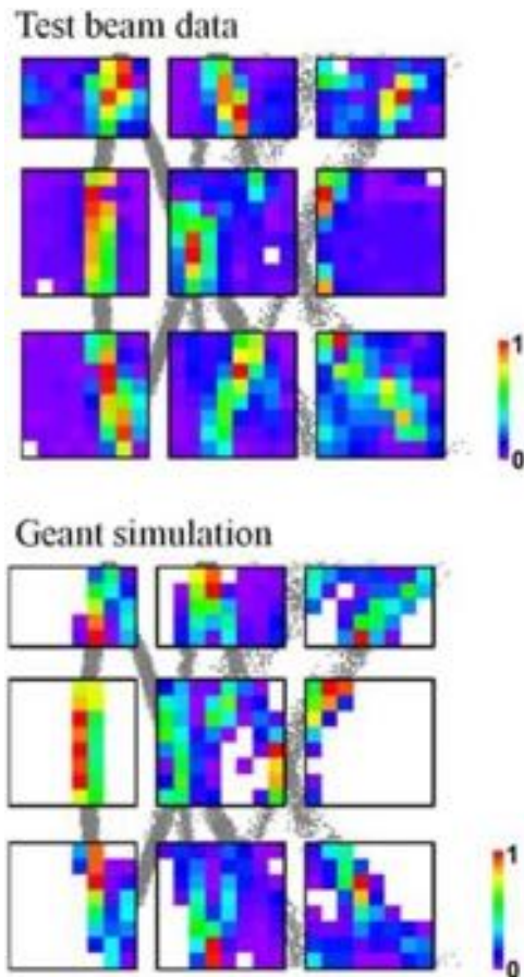
Figure 79. Cherenkov hit pattern from experimental data (top) and simulation (bottom) for the 2012 prototype. The normalized hit probability is shown for a spherical lens with air gap, a polar angle of 124^\circ and a beam momentum of 10 \text{ GeV}/c .
