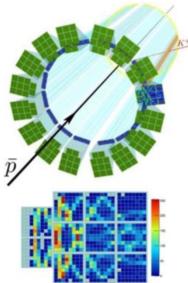
Figure 14. Geant simulation of the baseline geometry of the PANDA Barrel DIRC. The colored histogram at the bottom shows the accumulated hit pattern from 1000 K^+ at 3.5 GeV/c momentum and 55^\circ polar angle, the red line shows the kaon trajectory. (Top) Reproduced from 2018 JINST 13 C03004. © 2018 IOP Publishing Ltd and Sissa Medialab srl. All rights reserved. (Bottom) Reproduced from 2017 JINST 12 C07006. © 2017 IOP Publishing Ltd and Sissa Medialab srl. All rights reserved.
