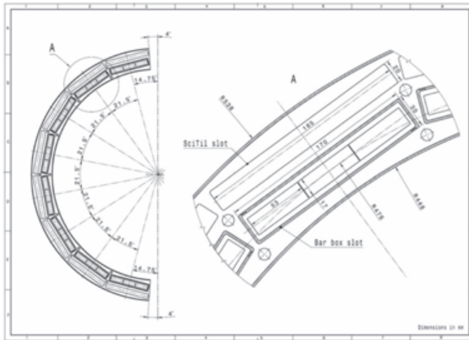
Figure 126. Sketch of a cross section of the radiator barrel with a zoom into the area covered by one bar box.
