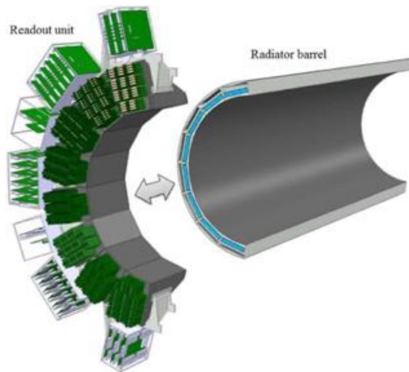
Figure 124. Mechanical design of the two main parts of the \bar{P} ANDA Barrel DIRC—half-section view: readout unit and radiator barrel. Reproduced from 2018 JINST 13 C03004. © 2018 IOP Publishing Ltd and Sissa Medialab srl. All rights reserved.
