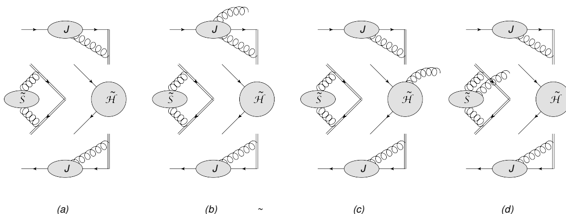
Figure 1. (a) Schematic factorisation of a two-point amplitude. \tilde{\mathcal{H}} and \tilde{\mathcal{S}} are the hard and next-to-soft functions, and J is a non-radiative jet function; next-to-soft subtractions to J are omitted for simplicity. (b) Emission of a gluon from a jet (to be described by a radiative jet function J^\mu ); (c) emission from the hard function. (d) Emission through a radiative next-to-soft function \tilde{\mathcal{S}}^\mu .
