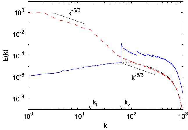
FIG. 5. Energy spectrum E^{2D}(k) of the 2D mode \mathbf{u}^{2D} (red, dashed line) and 3D mode \mathbf{u}^{3D} (blue, solid line). We also show the 2D spectrum of the vertically averaged vertical velocity u_z (black, dotted line). The spectra are computed at t = 100\tau_f .
