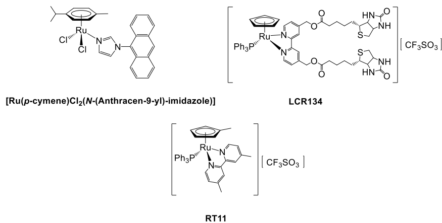
Figure 1. Ruthenium ABC pump inhibitors
