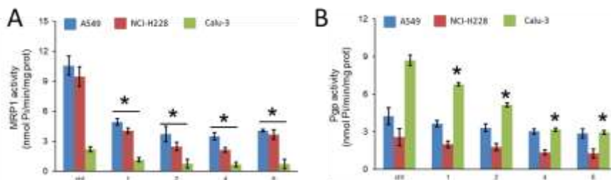
Figure 5. MRP1 (A) and P-gp (B) ATPase activity, measured spectrophotometrically on the proteins immune-purified from cells treated without (ctrl) or with 1 \mu M of compounds 1 , 2 , 4 and 6 for 24 h. Data are means \pm SD (n = 3). *p<0.05: vs ctrl.
