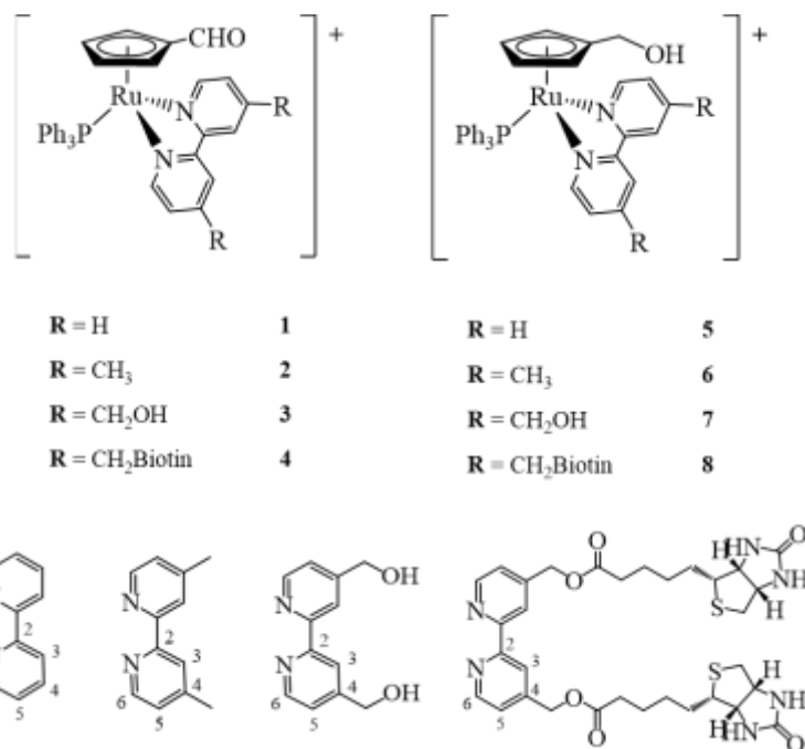
Figure 2. Chemical structures of compounds 1–8 . All compounds were isolated as \text{CF}_3\text{SO}_3^- salts.
