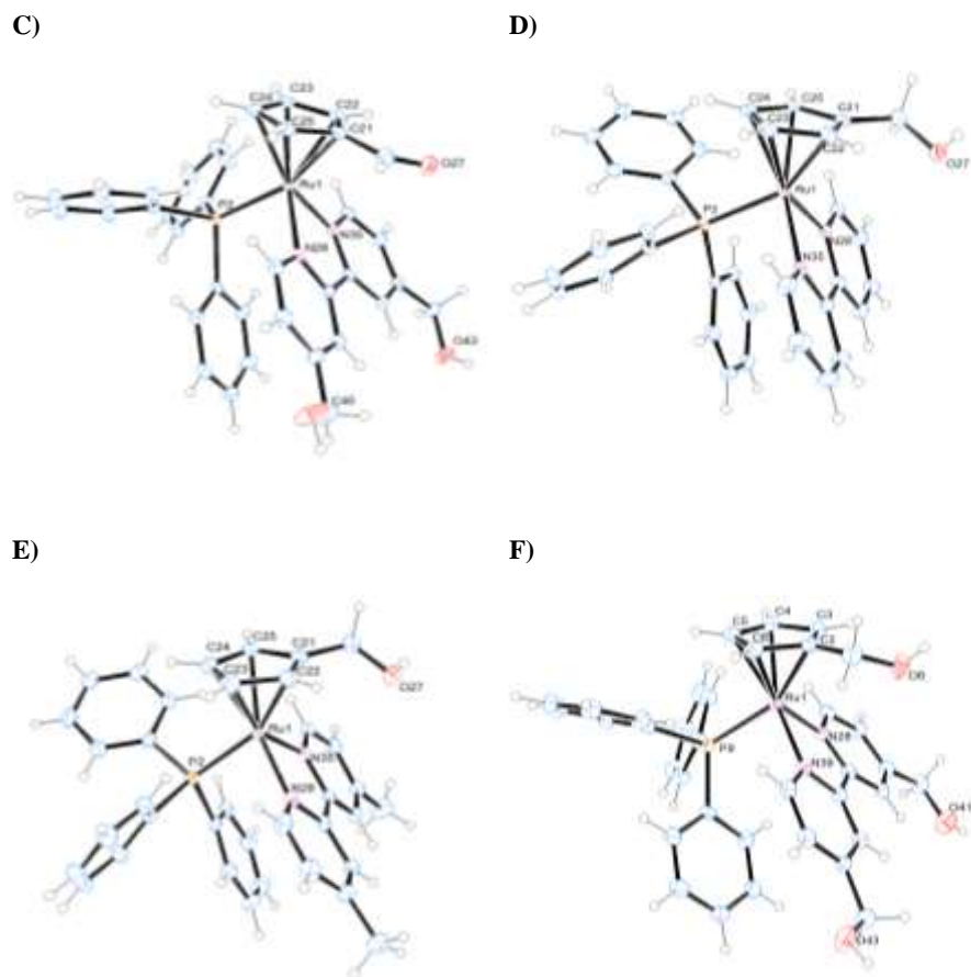
Figure 4. ORTEP plots and labeling schemes for the cations of complexes 1–3 (A–C) and 5–7 (D–F).
