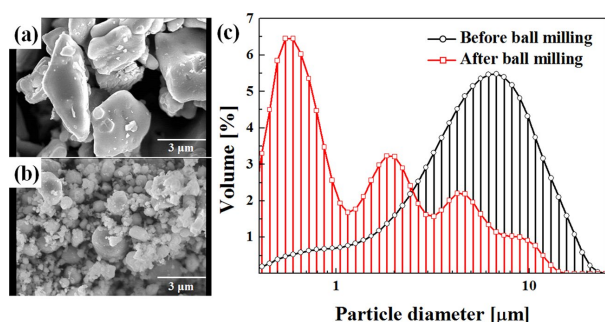
Figure 2. SEM images of Cu 2 O particles (a) before and (b) after 4 days of ball milling; and (c) particle size distribution of Cu 2 O particles from a laser-diffraction particle size analyzer before and after ball milling.
