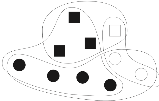
FIG. 3. Associative variables
