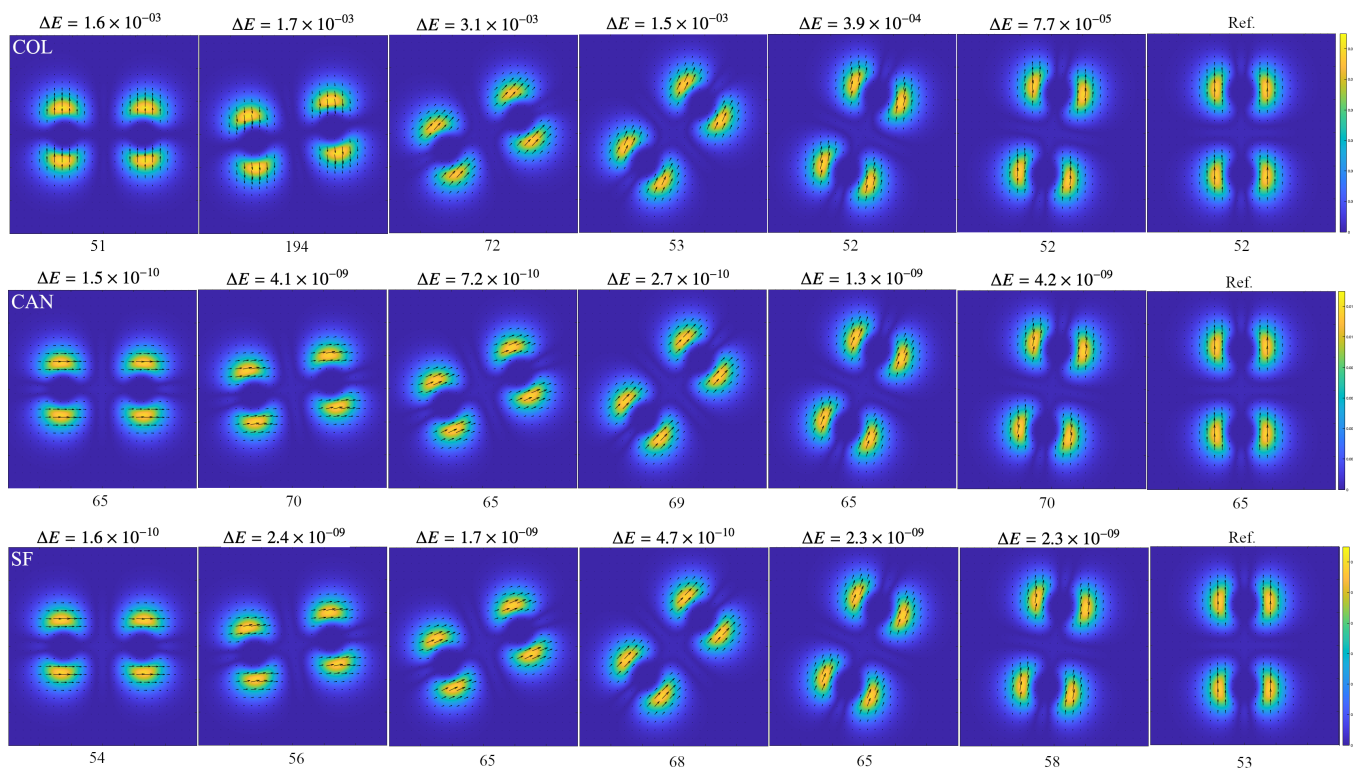
FIG. 1. Spatial distribution of the electronic magnetization for the I_2^+ molecule in the xz plane, as computed with the PBE xc functional, upon inclusion of SOC, with three formulations of the GGA theory: collinear COL, canonical CAN, and Scalmani-Frisch SF. The molecular axis and atomic guess magnetization is progressively rotated from the x axis (left) to the z axis (right). The small black arrows in the figure have lengths which reflect the magnitude and direction of the x and z components of the magnetization, while the color represents the magnitude m of the magnetization vector. The absolute value of the energy difference of each solution with respect to that obtained with the molecule along z is reported on top of the panels, as well as the number of cycles needed to converge the SCF, on the bottom of the panels. All quantities are reported in atomic units.
