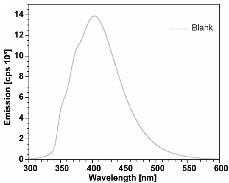
Figure S6. Emission spectrum of liquid BEDA without dyes or photoinitiator.
