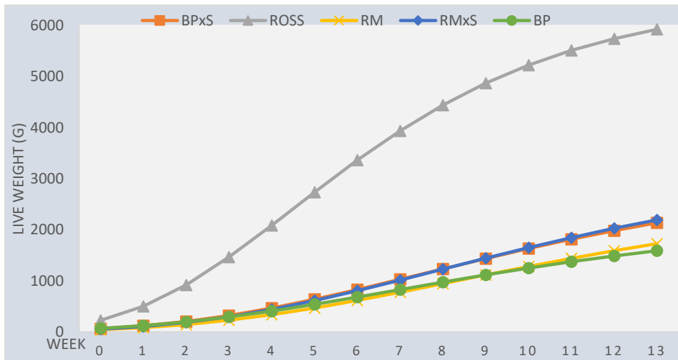
Figure 1. Gompertz distribution of LW from 0 to 13 weeks of industrial system.
