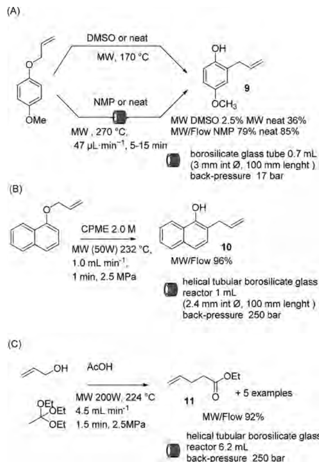
Scheme 5. Claisen Rearrangement
