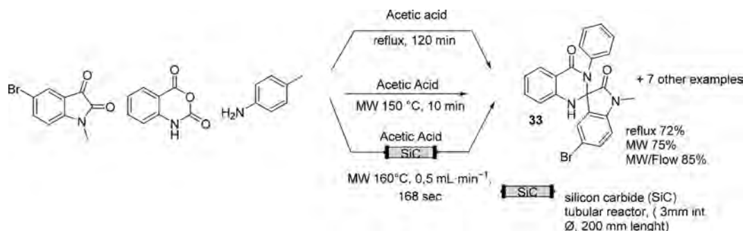
Scheme 19. Three-Component Spiro-Oxindole Synthesis
