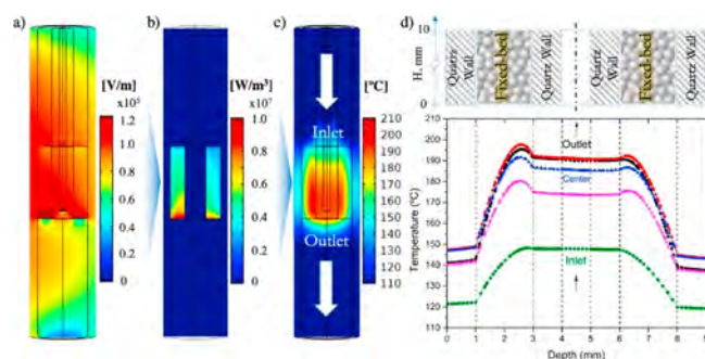
Figure 1. Simulated view of the quartz tube fixed bed of NaY zeolite and its corresponding (a) electric field, (b) power, and (c,d) spatial temperature distribution at steady state. Reproduced with permission from ref 13. Copyright 2019 Elsevier.
