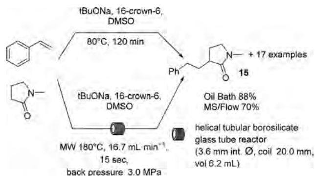
Scheme 7. C-Alkylation of N -Alkylamides
