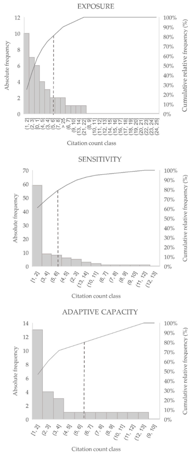
Figure 3. Pareto diagrams for the selection the of sub-indicators’ acceptance threshold. On the x-axis: citation count class (from the left, the least cited sub-indicators’ classes to the right, the more cited sub-indicators’ classes). On the y-axis: left ) absolute frequency; right ) cumulative relative frequency (%). The vertical dashed bar demarcates the 80–20% boundary.
