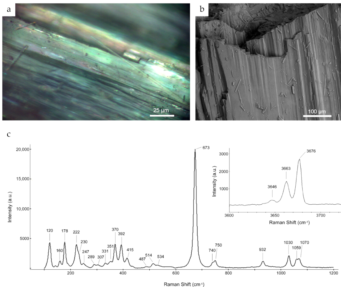
Figure 4. Sample #S3 (a) green columnar aggregates analyzed by \mu -Raman spectroscopy; (b) SE image showing the same fragment; (c) \mu -Raman spectra in the region 100–4000 \text{cm}^{-1} .
