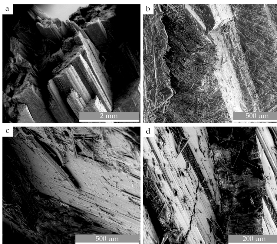
Figure 6. SE images of the asbestiform arrangement of fibers, with some randomly oriented regions at different magnifications. (a) Parallel fibers in a columnar arrangement. (b) Parallel and randomly oriented fibers. (c) Fibers that appear to be detaching from the bulk. (d) Fracture area with randomly oriented fibers and visible asbestiform fibers.
