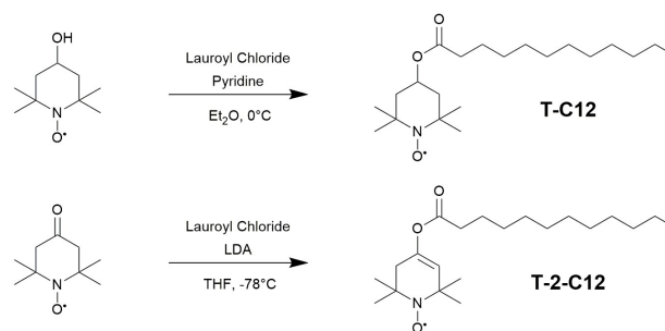
Scheme 1. Synthesis of Tempo-C12 (T-C12) and Tempo-2-C12 (T-2-C12).
