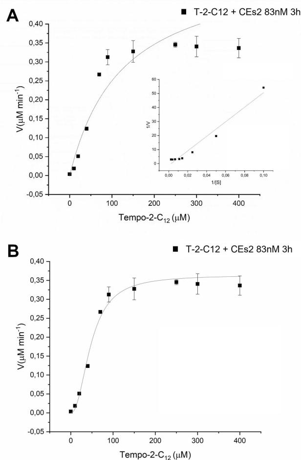
Figure 6. Enzymatic Kinetics of CE2 83 nM with T-2-C12 incubated for 3 h at 37 °C. Figure 6A shows the results fitted with the Michaelis-Menten equation and the Lineweaver–Burk plot, Figure 6B the fitting with the Hill equation.
