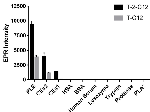
Figure 5. Selectivity assays of T-C12 and T-2-C12 200 μM with HSA, BSA, Lysozyme, Trypsin, Protease and PLA2 83 nM and Human serum (0.01 % dilution in HEPES-Buffered saline aqueous solution) incubated for 3 h at 37 °C.
