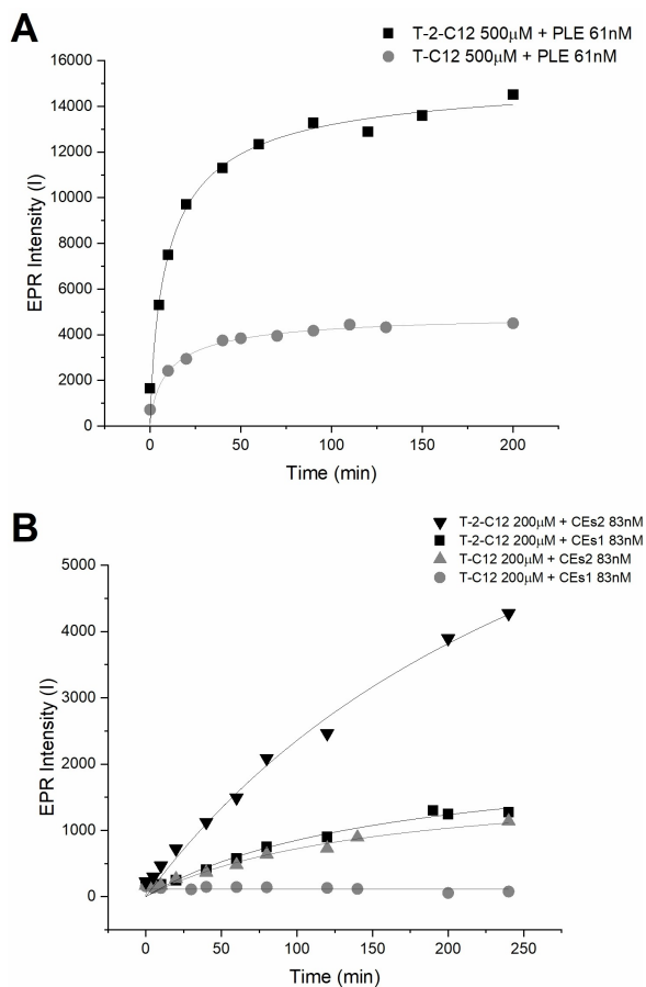
Figure 4. A) EPR signal intensity of T-C12 500 μM (gray curve) and T-2-C12 500 μM (black curve) incubated with PLE 61 nM from 0 to 200 minutes; B) EPR signal intensity of T-C12 200 μM (gray curve) and T-2-C12 200 μM (black curve) incubated with CE1 and CE2 83 nM at 37 °C from 0 to 240 minutes.
