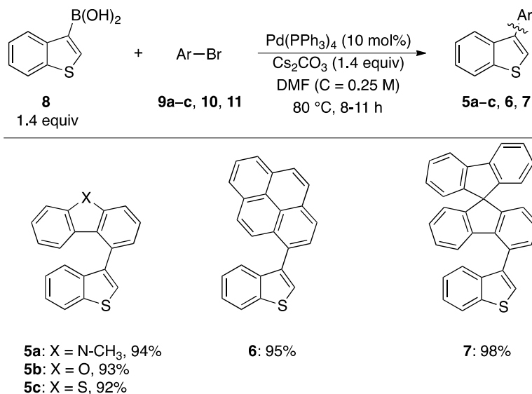
Scheme 1. Synthesis of bi(hetero)aryls 5a-c , 6 , and 7 .
