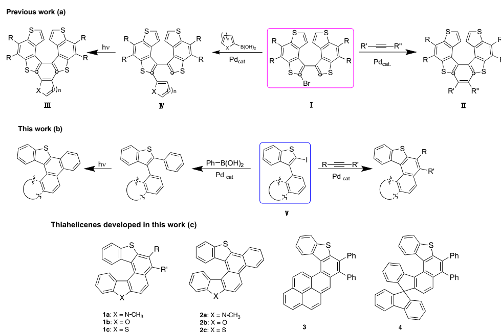
Figure 1. Synthetic strategies for the synthesis of 7-TH and novel thiahelices. (a) Previous work, (b) this work and (c) thiahelices developed in this work.
