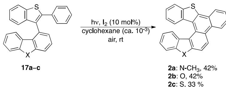
Scheme 5. Photocyclization of intermediates 17–19 .
