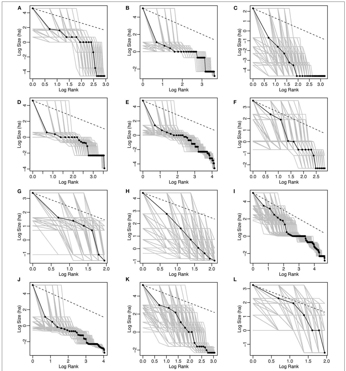
FIGURE 7 | Rank size for the territories of Iron Age/Orientalizing centres with sufficient data points. (A) Volterra, (B) Populonia, (C) Murlo, (D) Vetulonia, (E) Vulci, (F) Bisenzio, (G) Acquarossa, (H) Orvieto, (I) Tarquinia, (J) Cerveteri, (K) Veio, (L) Civita Castellana. The dark line represents the observed data. The grey lines represent the bootstrap results performed on random samples of sites.
