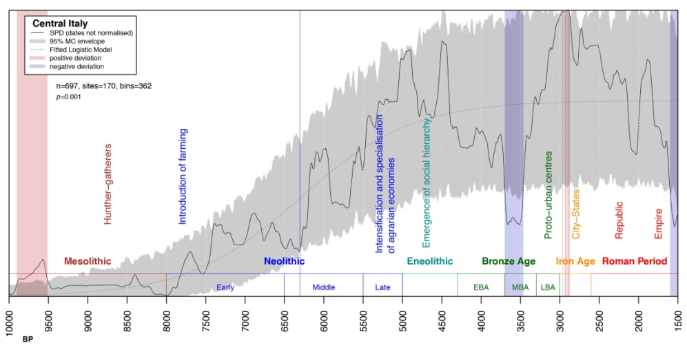
Fig. 2. Summed Probability Distribution (SPD) of unnormalised calibrated radiocarbon dates (solid line) vs. a fitted logistic model (95% Monte-Carlo confidence grey envelope) of population growth.
