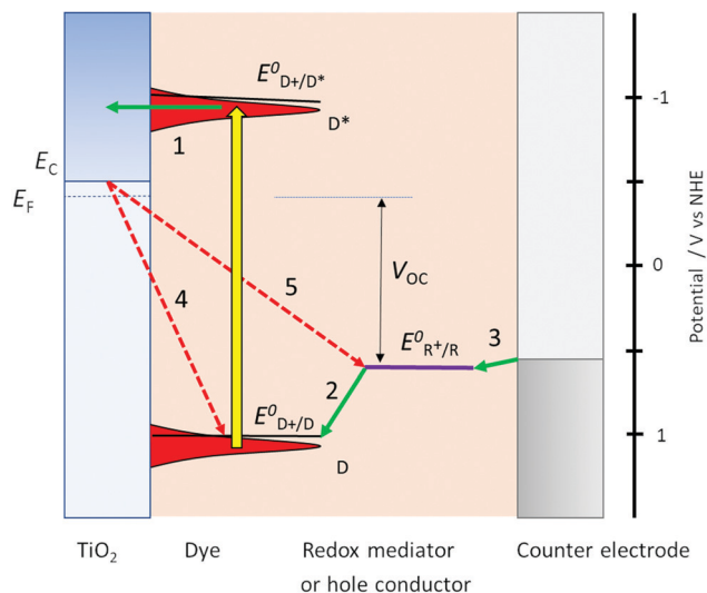
Fig. 3 Basic diagram of the dye-sensitized solar cell, displaying working mechanism and energy levels.
